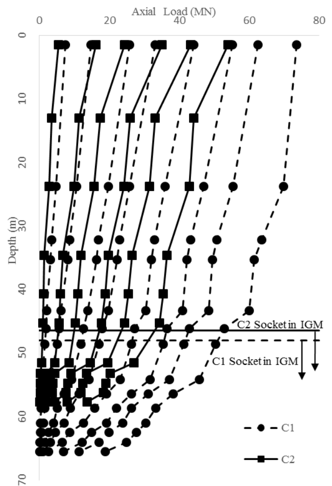
Figure 6 Load distribution of tested shafts C1 and C2
