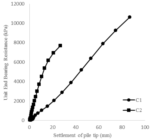
Figure 5 mobilized unit bearing versus settlement relationship of the Shafts C1 and C2
