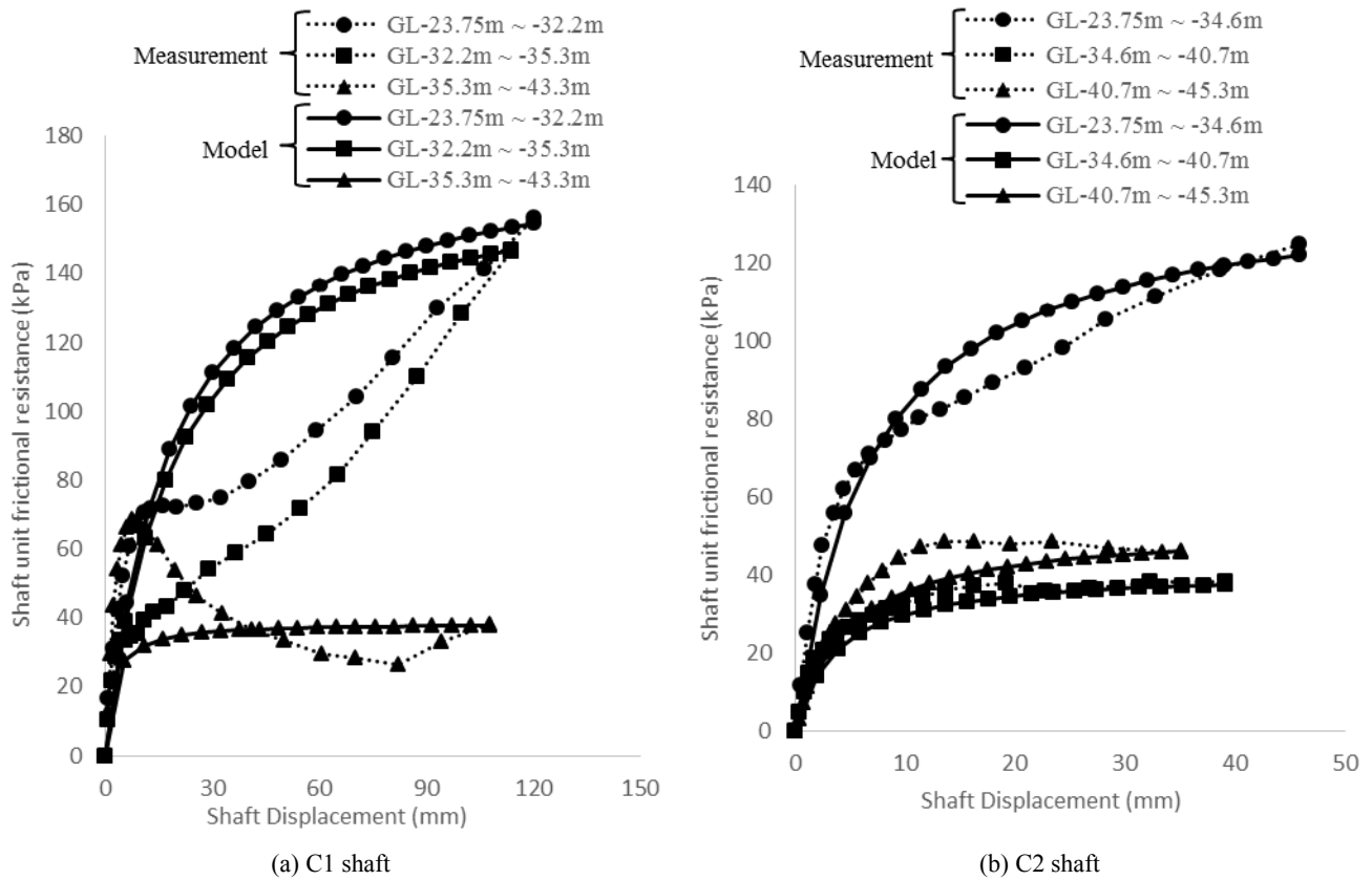
Figure 8 Hyperbolic model fitting of t-z curves in clay layer
