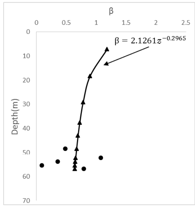
(b) C2 shaft
