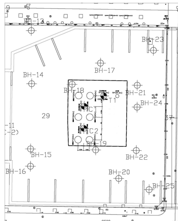
Figure 2 Location of C1 and C2 Shafts in the project
