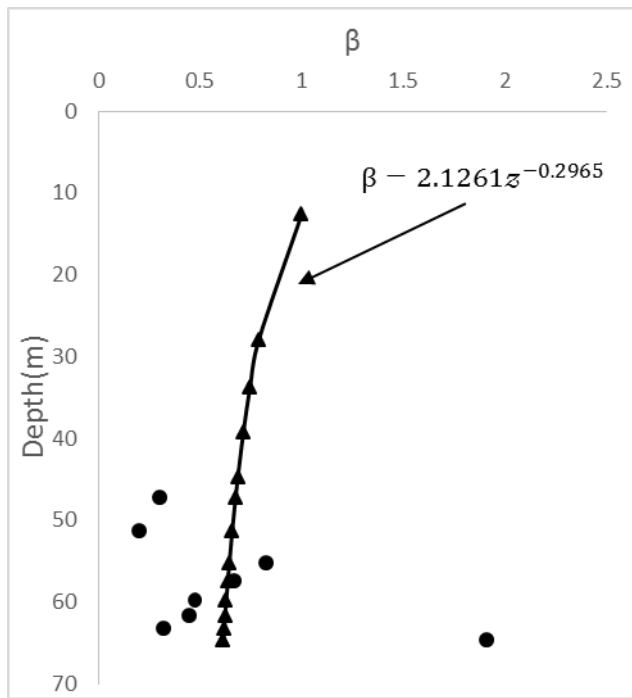
(a) C1 shaft
