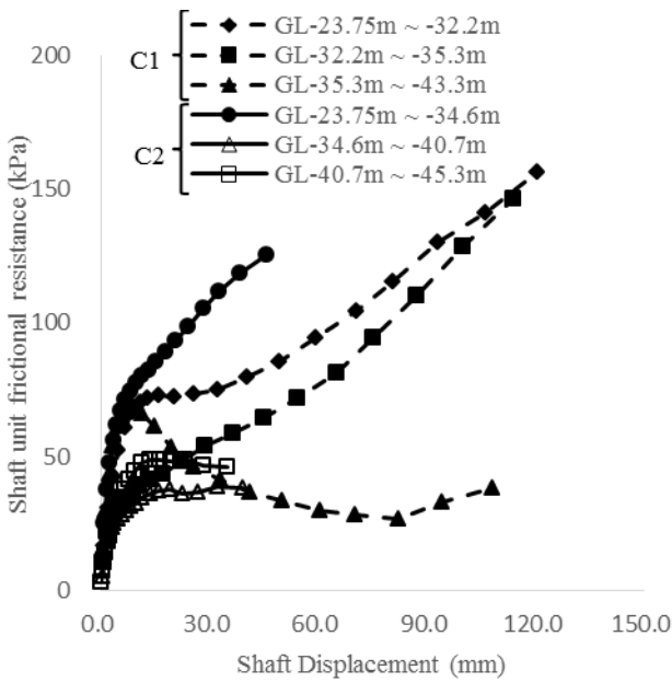
(a) Clay layer
