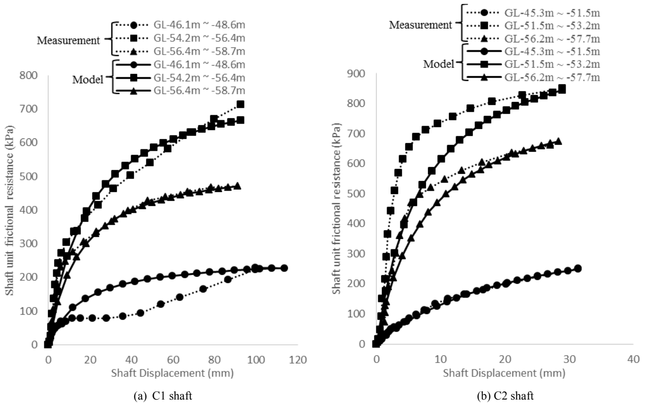
Figure 9 Hyperbolic model fitting of t-z curves in IGM layer
