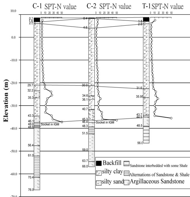
Figure 1 SPT-N Value in Soil and IGM
