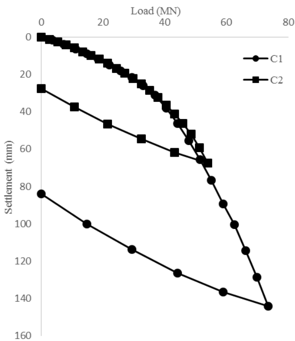
Figure 4 Pile head movement of the tests shafts C1 and C2
