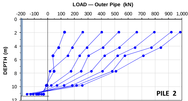
Figure 3A Force distribution in the outer pipe (data from Jeong and Ko 2015)
