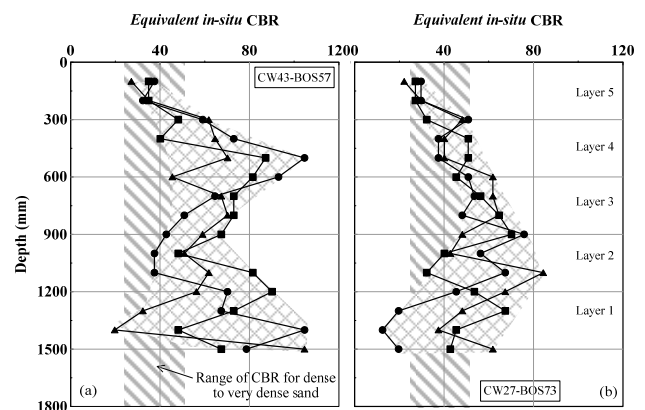
Figure 9 Variation of the equivalent in-situ CBR with depth for (a) CW43-BOS57 and (b) CW27-BOS73 (Tasalloti et al., 2015b)
