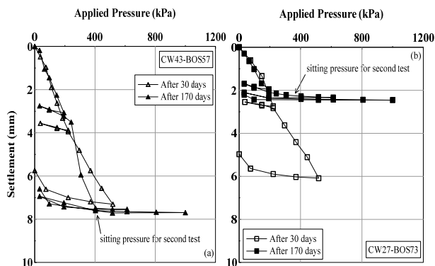
Figure 10 Variation of pressure against settlement on (a) CW43-BOS57 and (b) CW27-BOS73 (Tasalloti et al., 2015b)
