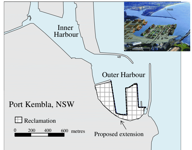
Figure 6 Illustration of the proposed extension area of the Port Kembla
