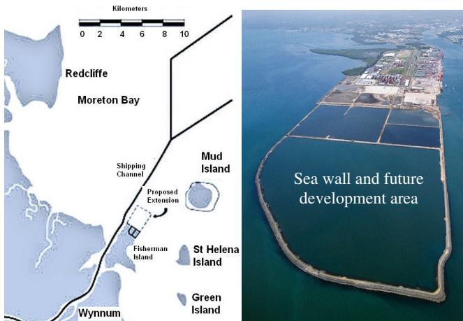
Figure 1 Illustration of the proposed extension area of the Port of Brisbane (modified after Indraratna et al., 2011)
