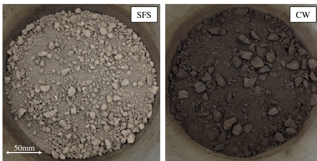
Figure 7 Typical aspect of steel furnace slag (SFS) and coal wash (CW) granular waste by-products
