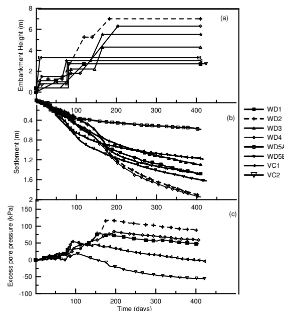
Figure 4 Embankment responses (a) staged construction, (b) settlements and (c) excess pore pressures (Indraratna et al., 2011)
