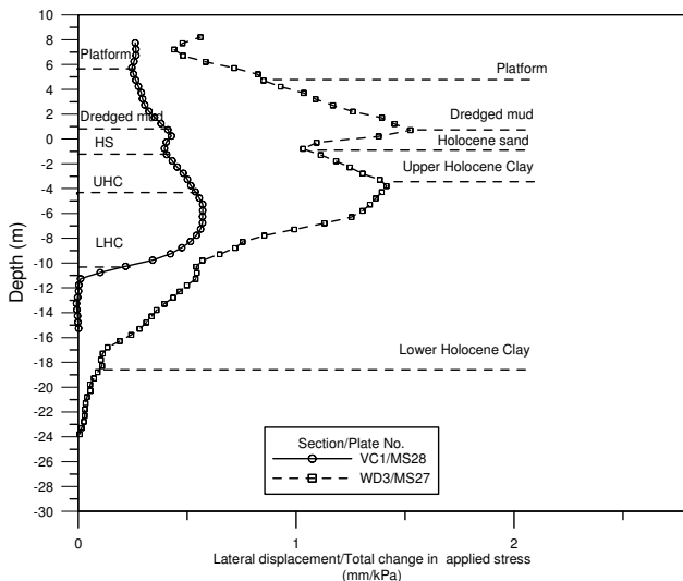
Figure 5 Comparison of lateral displacements at the embankment toe in vacuum and non-vacuum area after 400 days (Indraratna et al., 2011)
