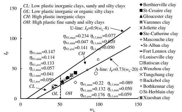
Figure 6 Classification of selected soils in plasticity chart
