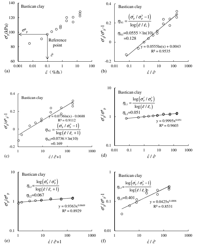
Figure 5 Comparison of pre-consolidation - rate formulations
