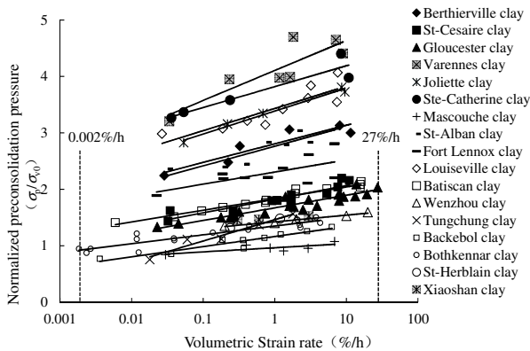
Figure 3 Pre-consolidation pressure versus applied strain-rate
