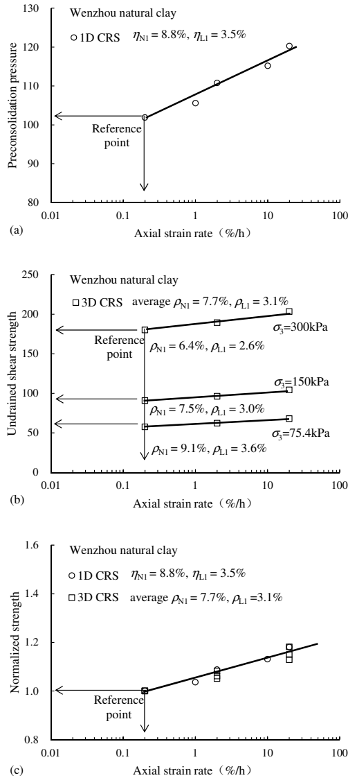
Figure 14 1D and 3D strain rate effect for Wenzhou clay
