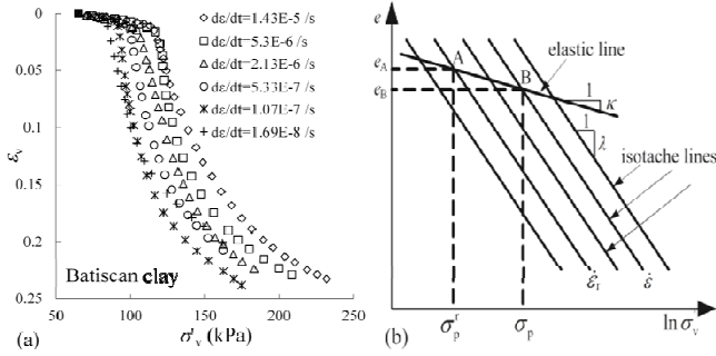
Figure 2 Stress-strain-strain-rate behavior of 1D CRS tests
