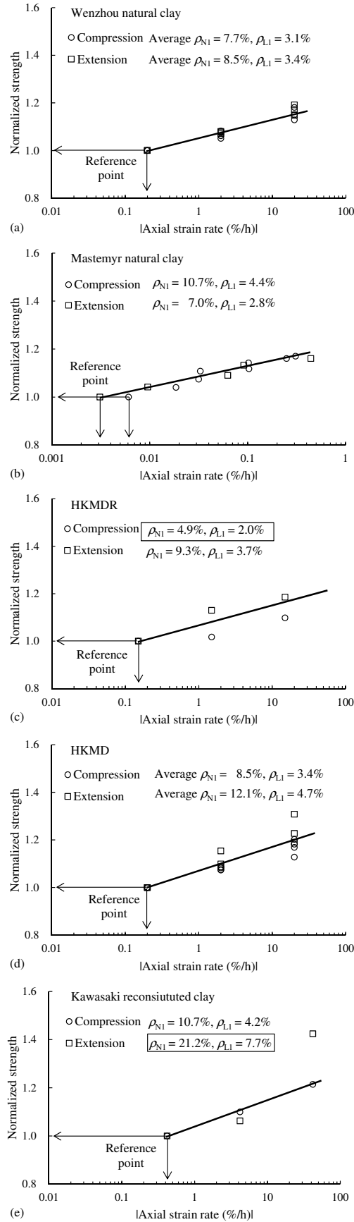
Figure 16 Normalized compression and extension strength versus axial strain rate
