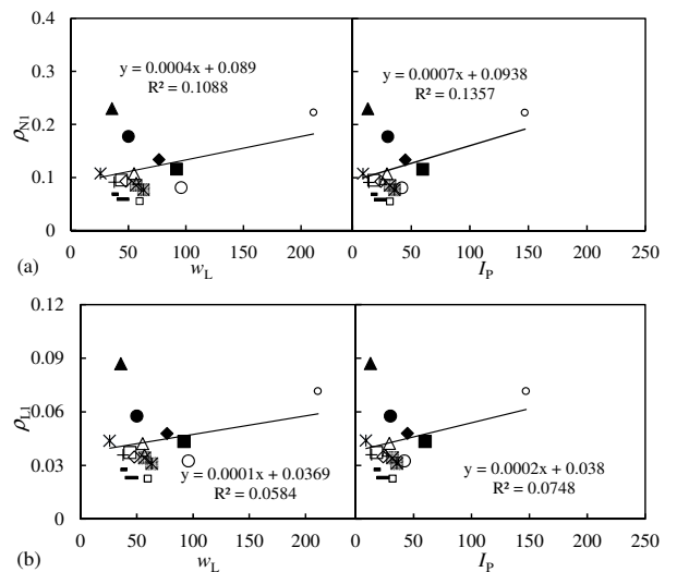
Figure 12 Relationship between \rho_{N1} , \rho_{L1} and w_L , I_p
