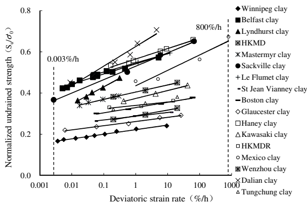
Figure 8 Relationship between Normalized undrained shear strength versus Deviatoric strain rate
