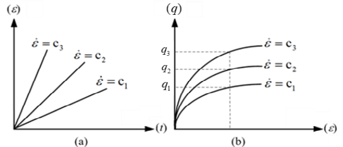
Figure 1 Schematic plot for CRS tests: (a) strain history; (b) stress-strain relationship
