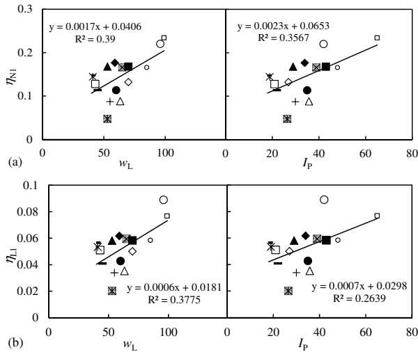
Figure 7 Relationship between rate parameters and liquid limit and plasticity index
