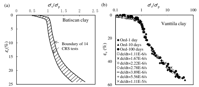
Figure 4 Normalized stress-strain relationship deduced from CRS tests
