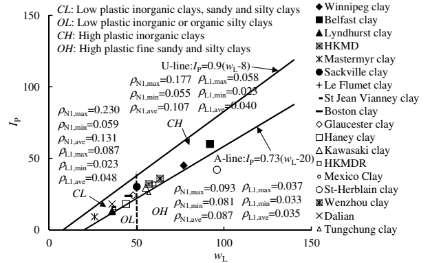
Figure 11 Classification of selected soils in plasticity chart
