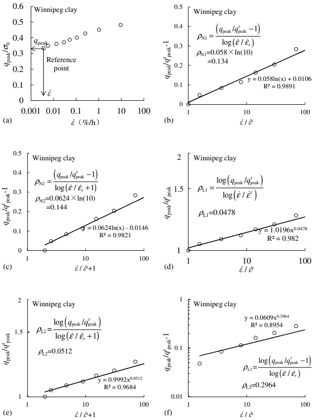
Figure 10 Comparison of rate formulation for triaxial undrained shear strength
