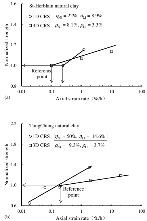
Figure 15 1D and 3D rate effect for St-Herblain and Tungchung clays
