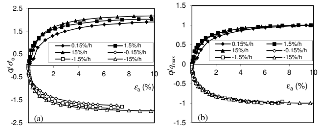
Figure 9 Normalized stress strain relationship for triaxial CRS compression and extension tests: (a) Normalized deviatoric stress by confined pressure versus axial strain; (b) Normalized deviatoric stress by maximum values versus axial strain
