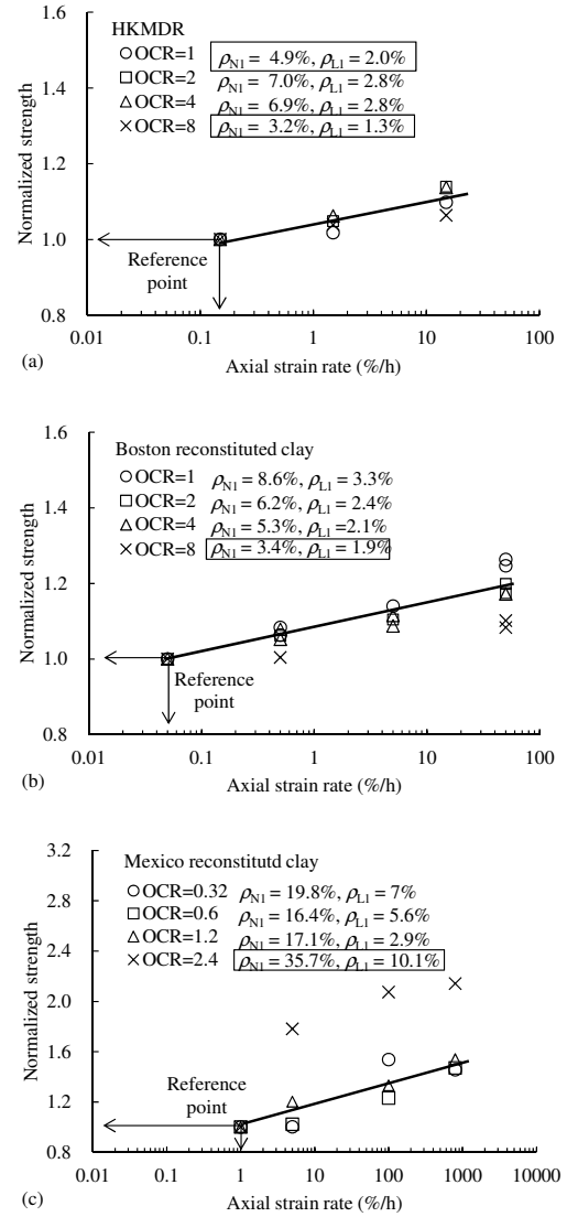
Figure 17 Normalized compression strength versus axial strain rate for different OCRs
