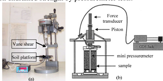
Figure 13 (a) Vane shear apparatus of laboratory; (b) Modified pressio-triax apparatus
