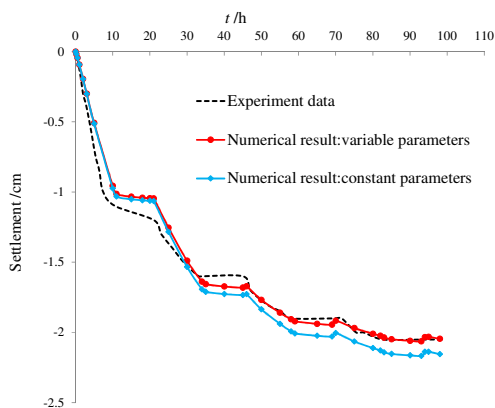
Figure 7 Surface settlement from experiment and numerical simulation (T2)
