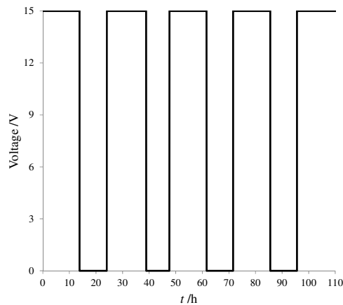
Figure 2 Applied voltage to the soil samples
