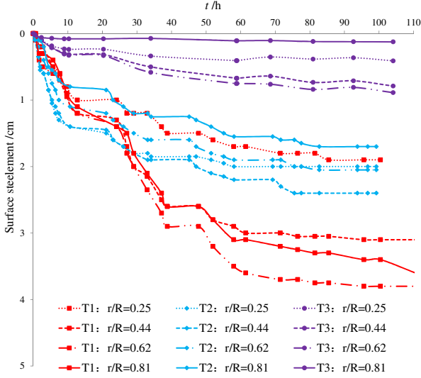
Figure 5 Surface settlement during electro-osmosis
