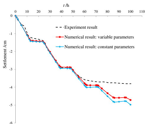
Figure 6 Surface settlement from experiment and numerical simulation (T1)
