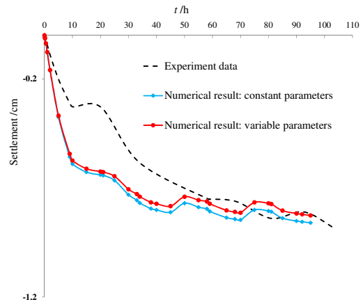
Figure 8 Surface settlement from experiment and numerical simulation (T3)
