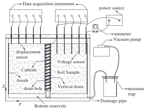
Figure 1 Axisymmetric model for electro-osmosis experiment
