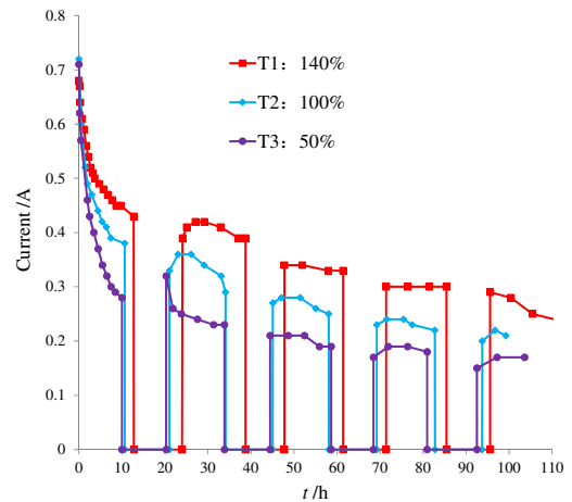
Figure 4 Current change during electro-osmosis
