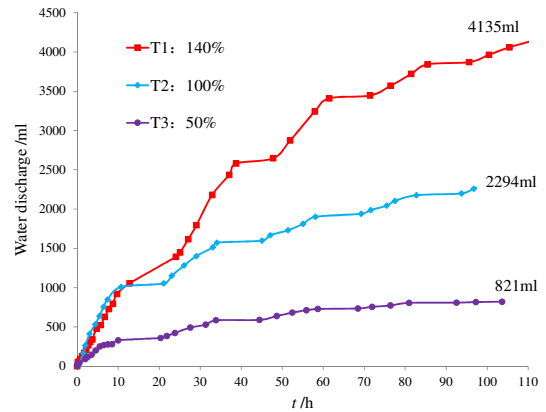
Figure 3 Water discharge during electro-osmosis
