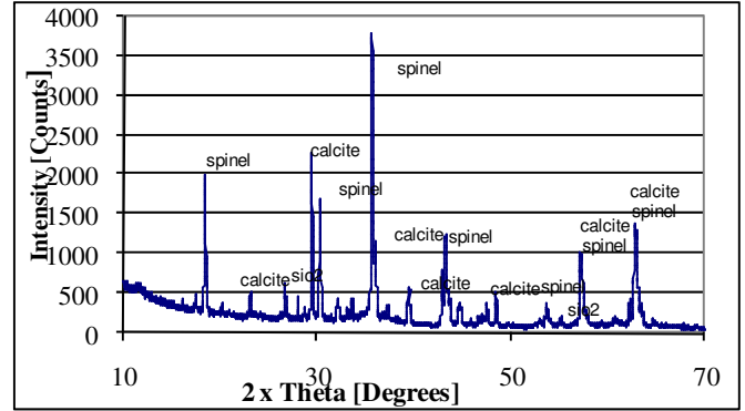
Figure 4 XRD Results of Chromium Contaminated Soil from LSP Site
