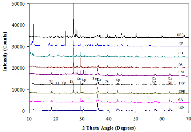
Figure 1 XRD results of Chromium Contaminated Soils from Nine Sites
