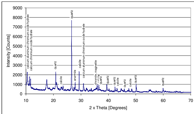
Figure 2 XRD Results of Chromium Contaminated Soil from CD Site
