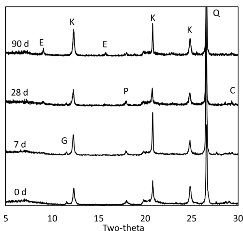
Figure 6 XRD patterns of quartz-kaolinite blend stabilized with 5% lime, 1% corundum and 3% anhydrite at 0, 7, 28 and 90 days curing (Q: Quartz, K: Kaolinite, C: Calcite, P: Portlandite, G: Gypsum, E: Ettringite)
