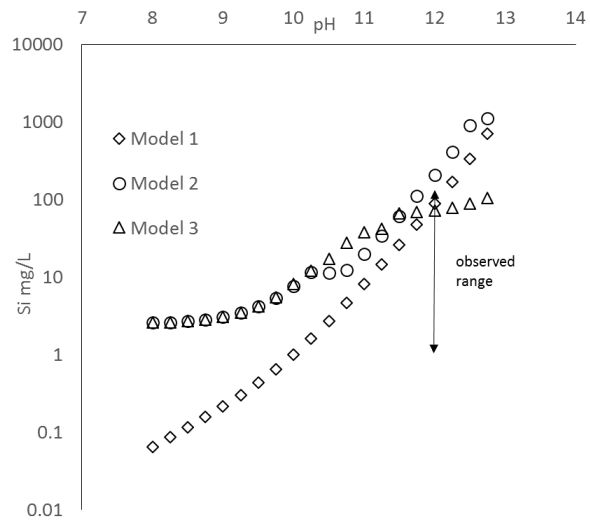
Figure 4 Total dissolved Si in three modeling scenarios
