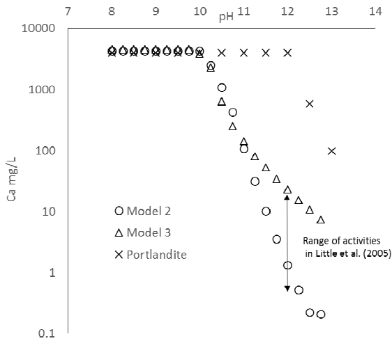
Figure 3 Total dissolved \text{Ca}^{2+} in two modeling scenarios and in equilibrium with portlandite
