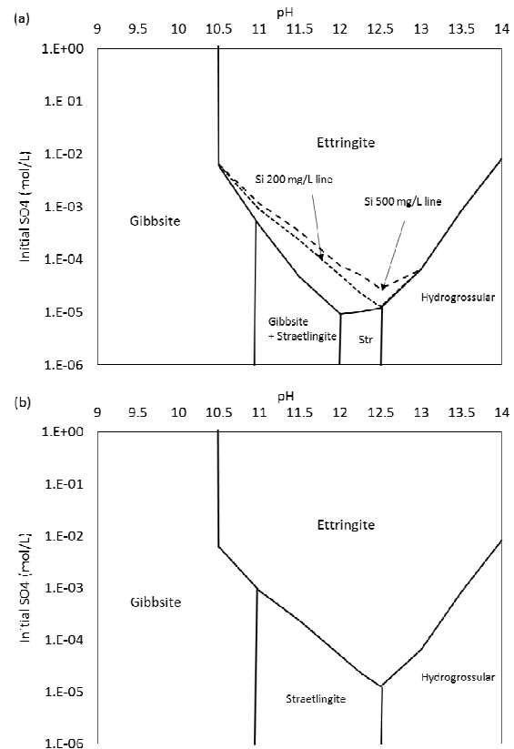
Figure 5 Thermodynamic phase diagrams for worst-case scenario and two Si concentrations (a) 10 mg/L (b) 200 mg/L
