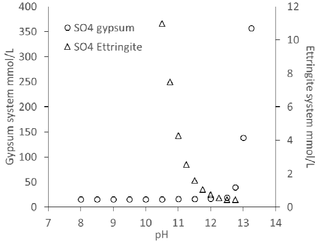
Figure 1 Modeled SO 4 2- concentrations in equilibrium with a solution containing only gypsum and only ettringite
