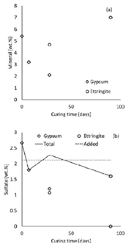
Figure 7 Gypsum and ettringite concentrations quantified in the XRD patterns of Figure 6
