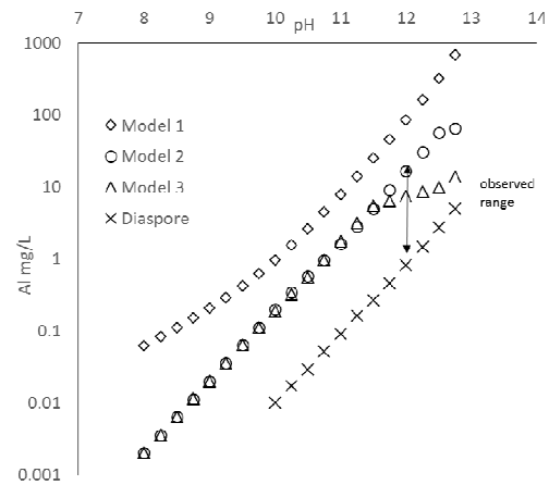
Figure 2 Total dissolved Al 3+ in three modeling scenarios and in equilibrium with diasporite
