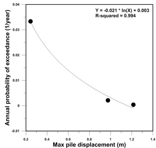
Figure 9 PBEE analysis on maximum pile displacement from EQWEAP for case study No.1
