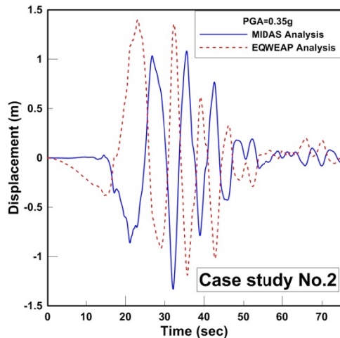
Figure 12 Displacement time history obtained from different analyses for P2 pile in case study No.2
