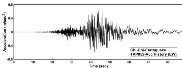
Figure 7 Acceleration time-history used in case study No.1
