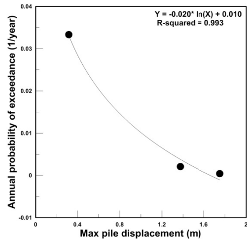
Figure 13 PBEE analysis on maximum pile displacement from EQWEAP for case study No.2
