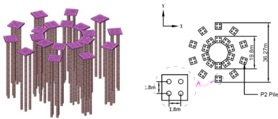
Figure 10 FE layout and bird view of the pile foundations in case study No.2
