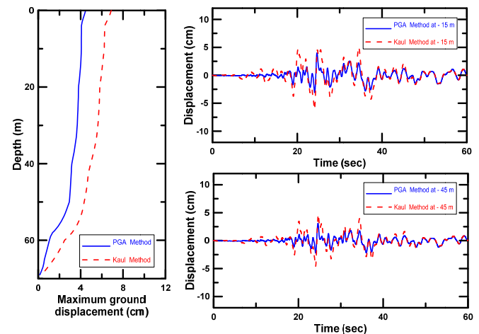
Figure 5 Comparisons of the ground displacements induced by artificial earthquakes
