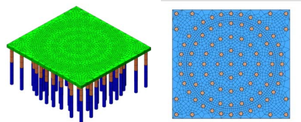
Figure 6 FE layout of pile raft foundation in case study No.1
