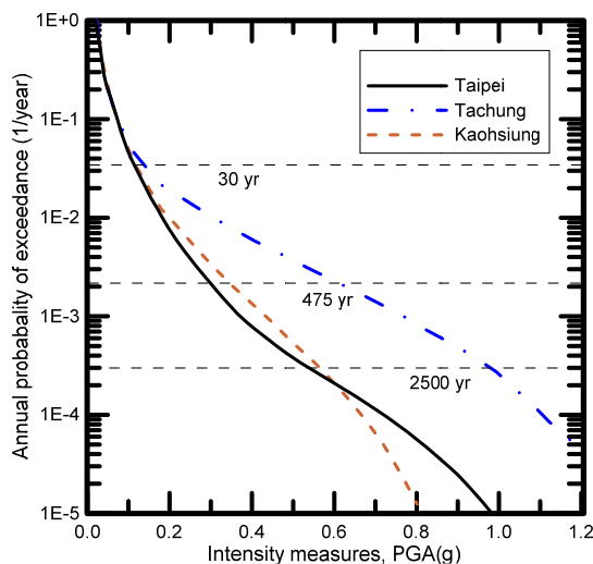
Figure 4 Seismic hazard curves suggested in Taiwan (Cheng, 2002)
