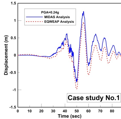
Figure 8 Displacement time history obtained from different analyses for P1 pile in case study No.1
