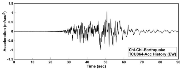
Figure 11 Acceleration time history used in case study No.2
