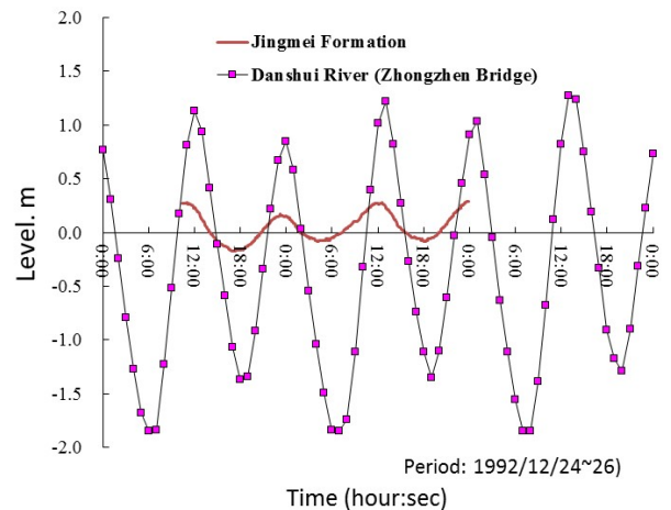
Figure 12 Piezometric levels in the Jingmei Formation as affected by tides (Shau, et al., 1995)
