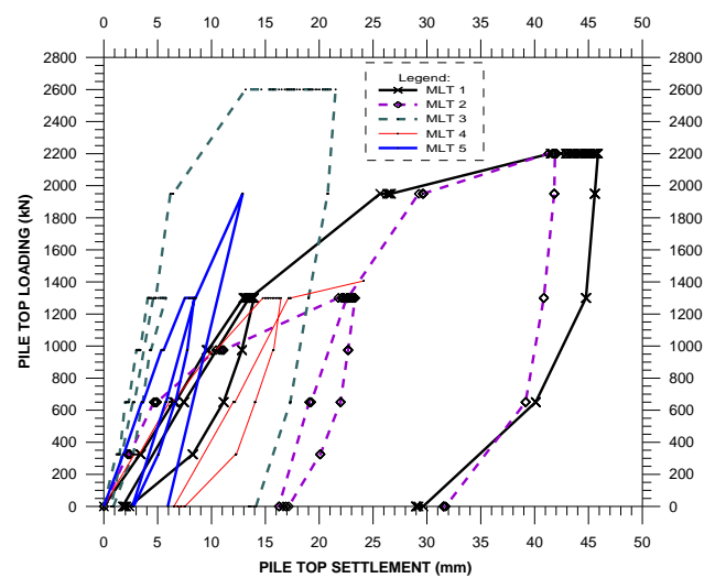
Figure 15 Pile top loading versus pile top settlement for contractually scheduled MLT results
