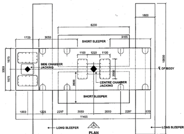
Figure 2 Typical plan view details of jack-in rig
