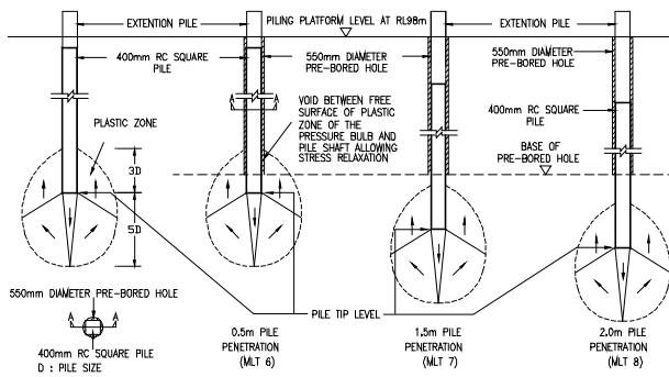
Figure 17 Schematic diagram of stress relaxation effect with relative position of pre-bored hole and pile stress bulb
