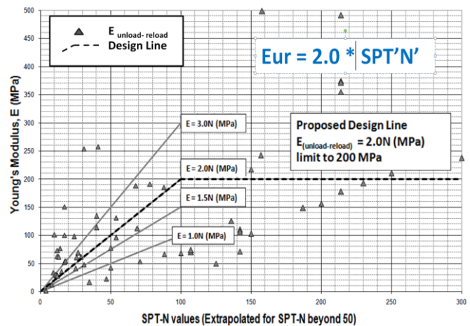
Figure 6 E_{ur} versus SPT 'N' plot of Kenny Hill Soils
