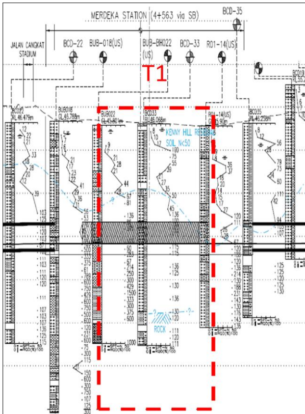
Figure 2A Merdeka Station boreholes layout
