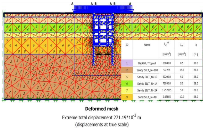
Figure 11 Bukit Bintang Station - Plaxis Meshing Model
