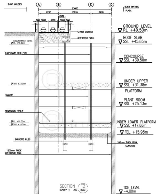
Figure 5A Bukit Bintang Station Cross Section T2
