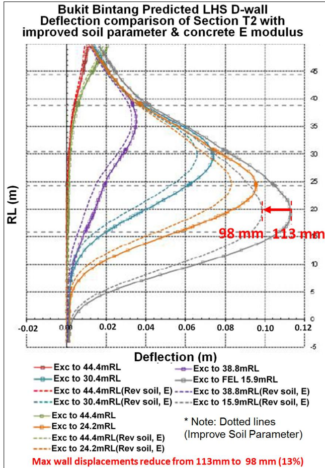
Figure 19 Comparison of displacement using better parameters versus design parameters (moderately conservative)
