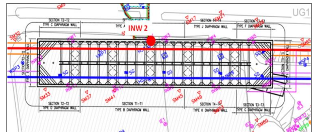
Figure 14 Merdeka in-wall Inclinometer INW2 for T1 D-wall
