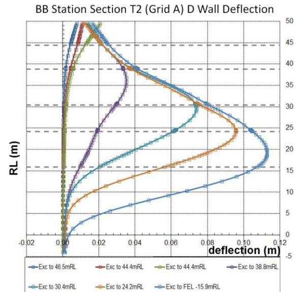
Figure 13 Bukit Bintang Station - Analysed Displacement Profiles at Various Stages
