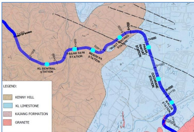
Figure 1 KVMRT alignment with underground stations superimposed on the Geology Map of Kuala Lumpur (1993)
