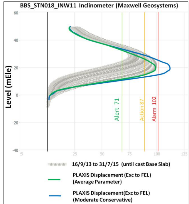
Figure 18 Displacement profiles from Inclinator INW11 Bukit Bintang T2 D-wall panel, taken from the project online data management system Maxwell geosystems' Mission OS Portal
