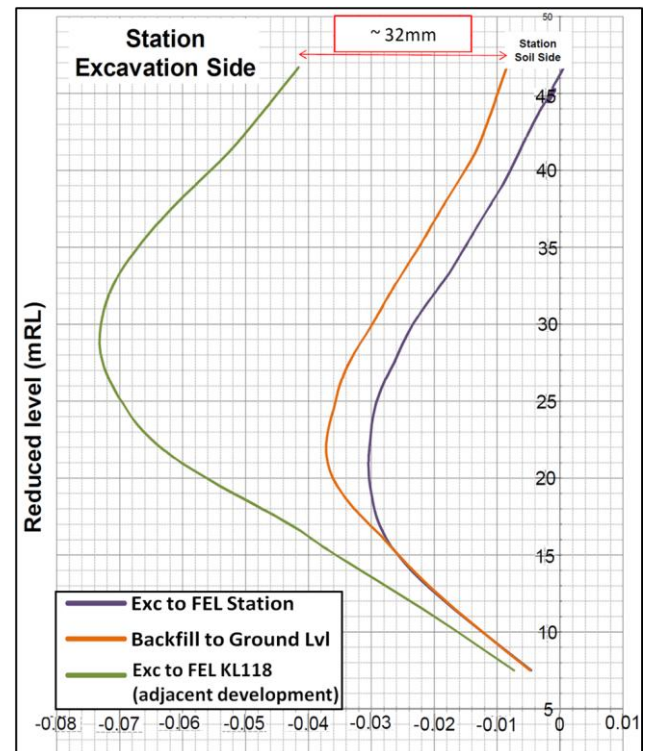
Figure 10 Merdeka Station - Analysed displacement Envelopes
