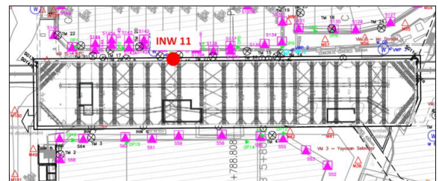
Figure 15 Bukit Bintang in-wall Inclinometer INW11 for T2 D-wall
