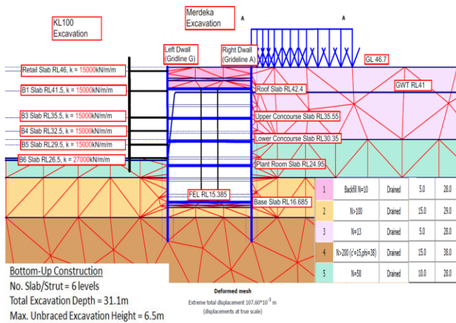
Figure 8 Merdeka Station - Plaxis Meshing Model.
