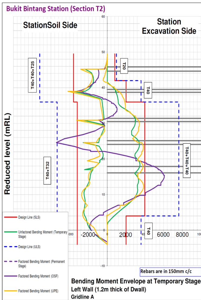
Figure 12 Bukit Bintang Station - SLS Bending Moment Envelope (Shops Side)
