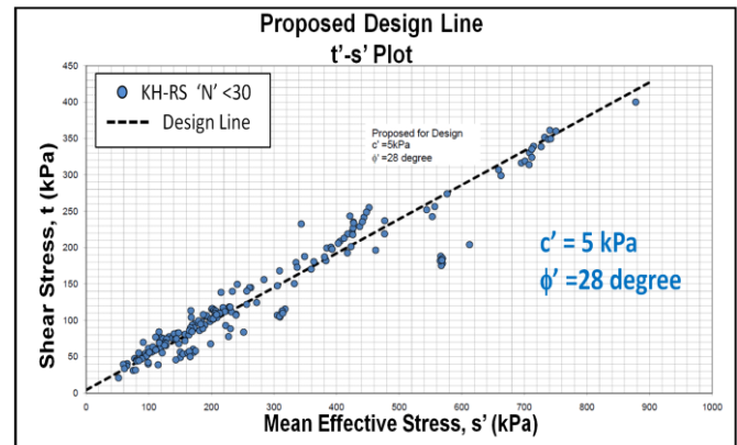
Figure 5 Shear Strength versus Mean Effective Stress plot of Kenny Hill SPT 'N' \leq 30 Soil
