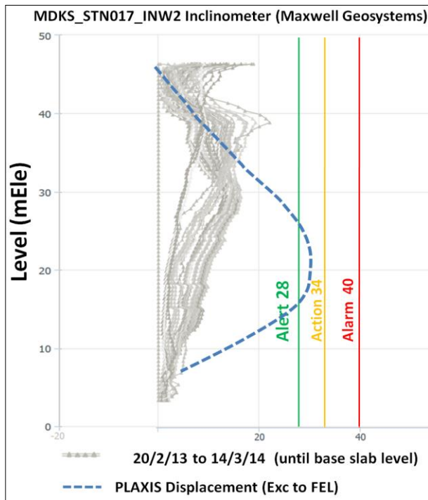
Figure 16 Displacement profiles from Inclinator INW2 Merdeka T1 D-wall panel
