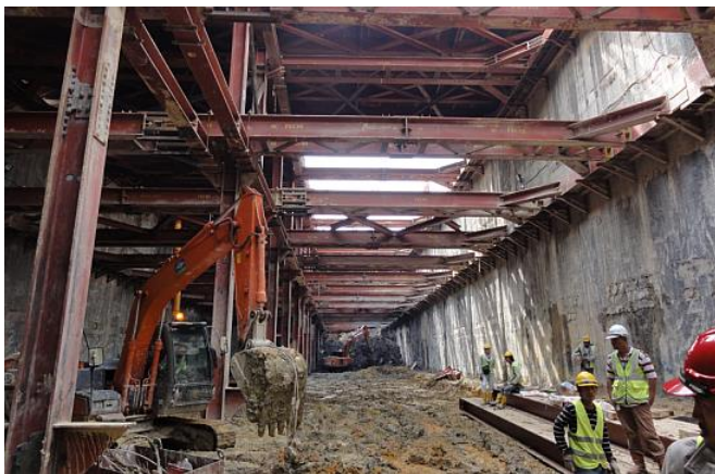
Figure 17 Bottom up excavation at the Merdeka Station
