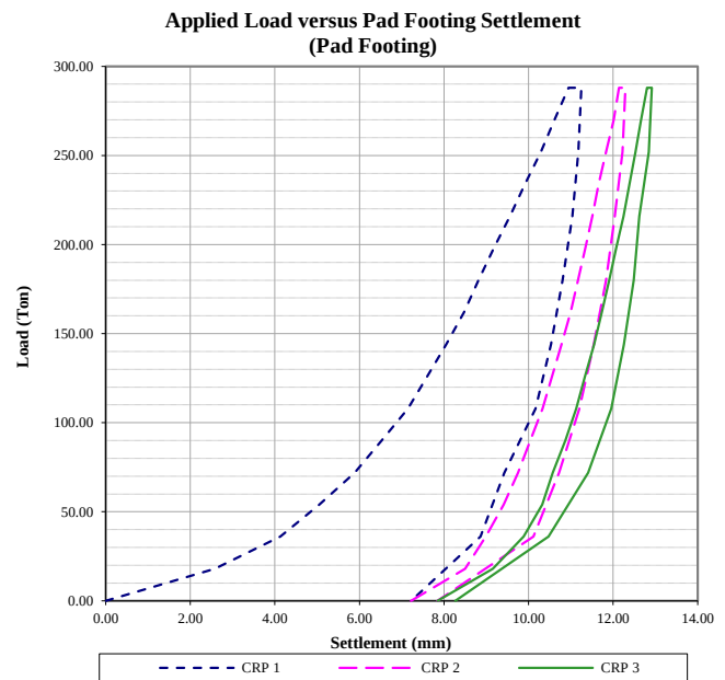
Figure 11 Load-settlement behaviour of pad footing
