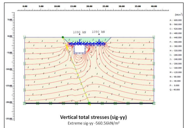
Figure 14 Finite element model with presence of cavity
