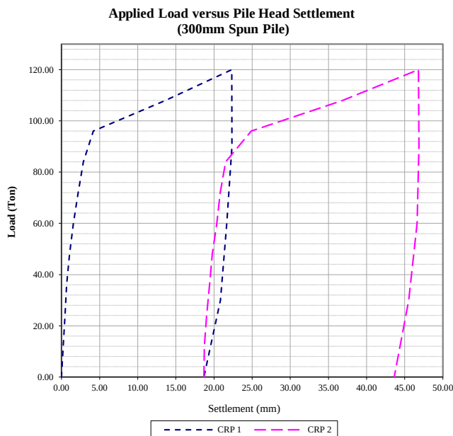
Figure 9 Load-settlement behaviour of 300mm spun pile
