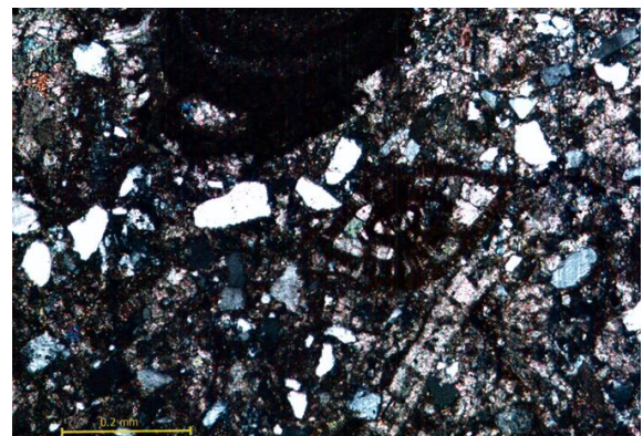
Figure 1 Petrographic thin section of hardpan calcrete
