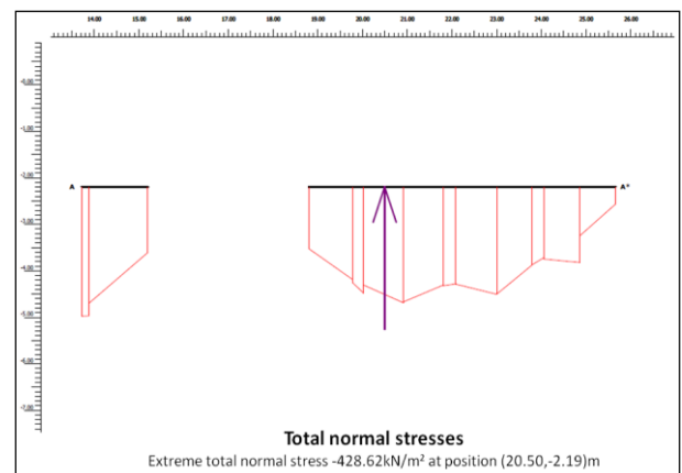
Figure 15 Analysed stresses acting on pad footing considering presence of cavity
