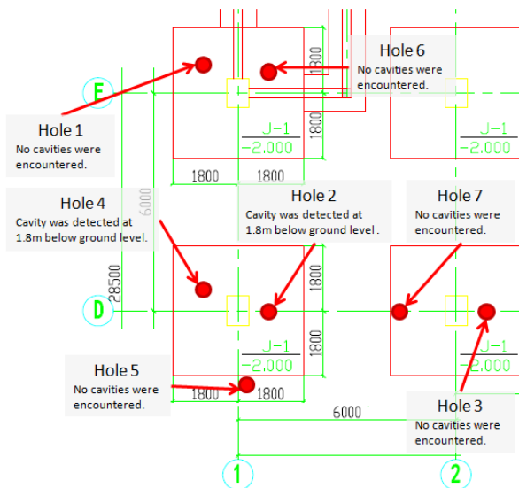
Figure 12 Investigation holes performed to verify presence of hardpan calcrete
