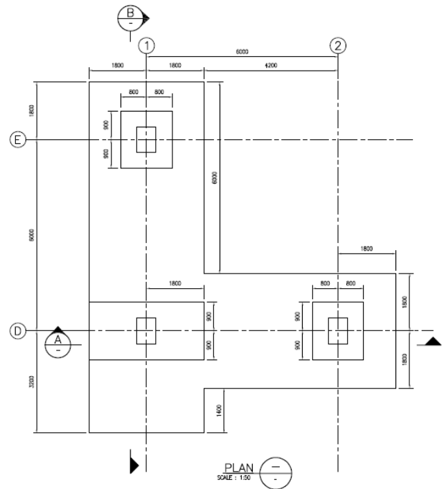
Figure 13 Re-designed combined pad footings
