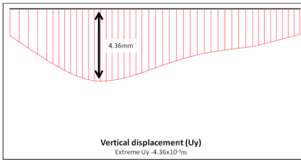
Figure 16 Analysed settlement considering presence of cavity
