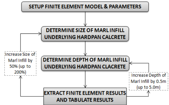
Figure 17 Procedure to analyse shallow foundation on hardpan calcrete with underlying marl infill
