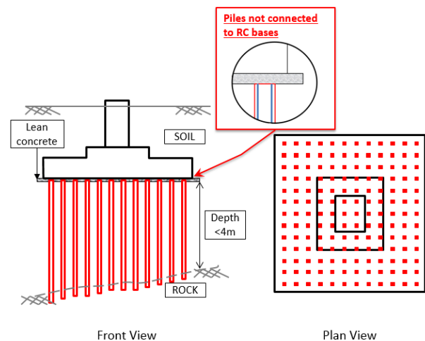
Figure 20 Schematic of 'pile-supported' pad footing for ground with overburden less than 4m
