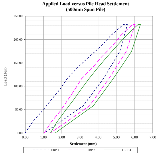
Figure 10 Load-settlement behaviour of 500mm spun pile
