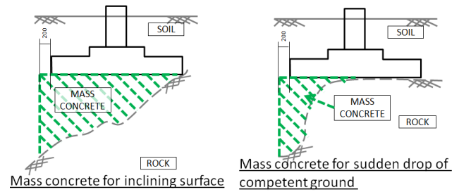
Figure 19 Schematic of mass concrete for pad footing supported on undulating rock profile
