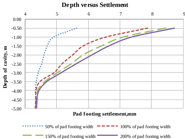
Figure 18 Analyzed relationships between depth of cavity and settlement of pad footing
