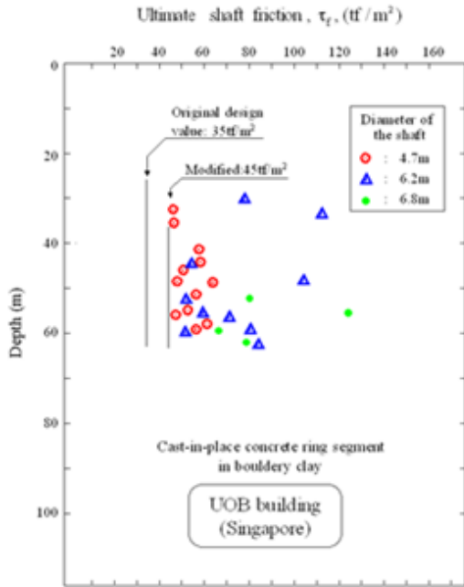
Figure 31 Ultimate shaft friction obtained from the in-situ loading tests
