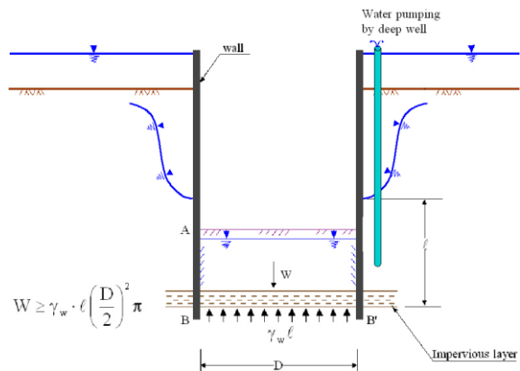
Figure 38 Stability against bottom uplift
