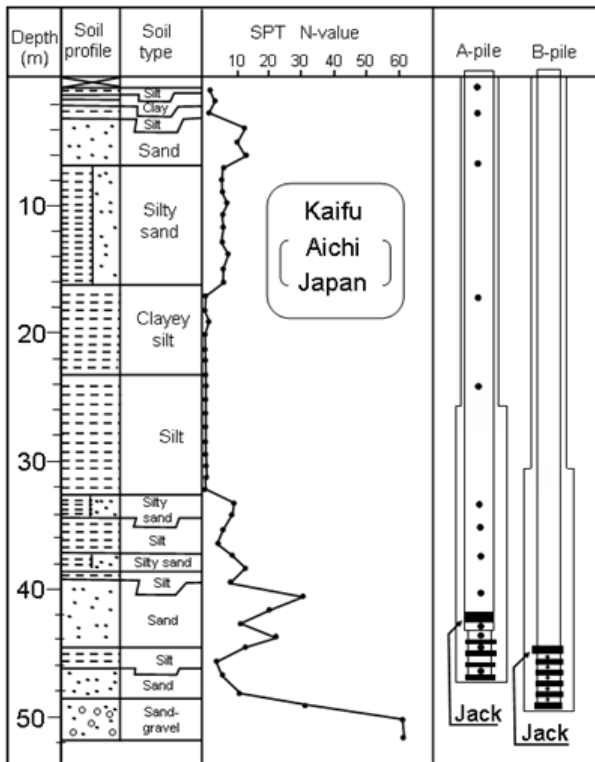
Figure 10 Soil profile at Kaifu site and embankment of two piles for piles for toe bearing and skin friction tests (Ogura et al , 2005)
