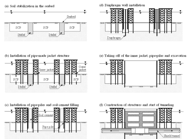
Figure 46 Construction process of the man-made Island
