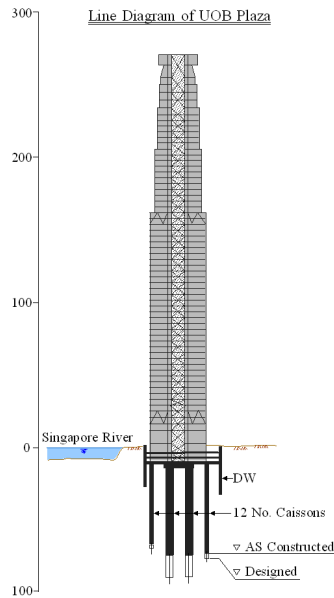
Figure 22 UOB Plaza in Singapore
