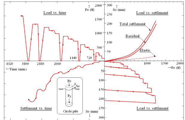
Figure 18 Load-settlement-time relations obtained by the pile top loading test on circular pile, Tsukimino, Kanagawa (Iwanaga et al. 1991)
