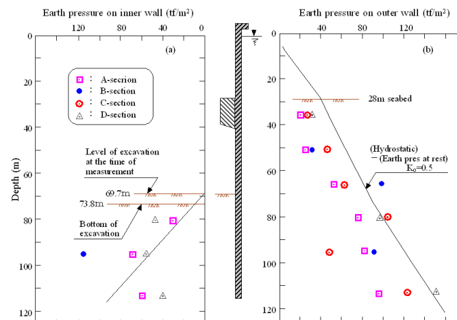
Figure 55 Measured earth pressure at two locations around the diaphragm wall
