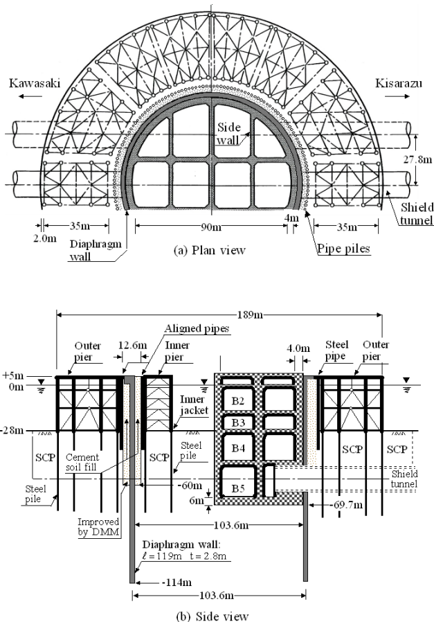
Figure 48 Layout of the platform and piers in Kawasaki Island
