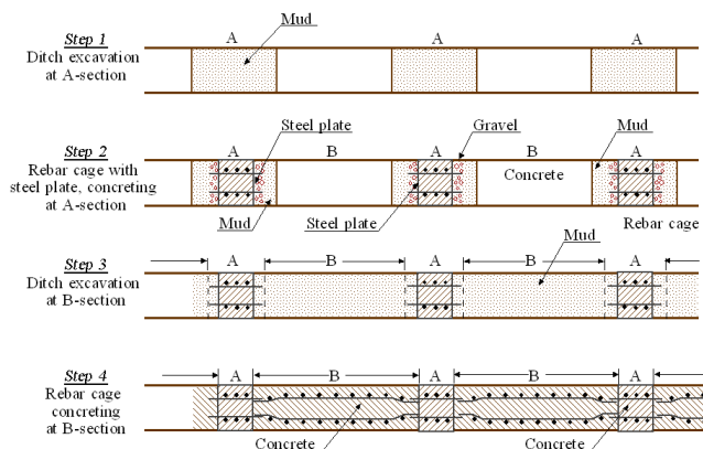
Figure 39 Diaphragm wall by rebar lapping method
