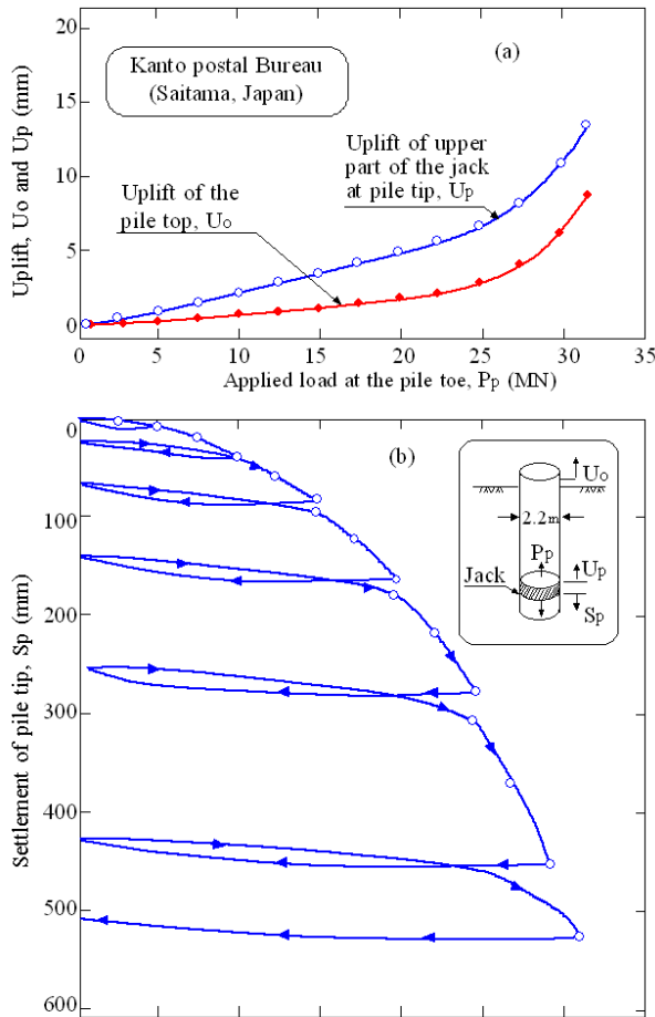
Figure 4 Results of the pile toe loading test at the site of Kanto Postal Bureau (Shibuya et al. 1997)
