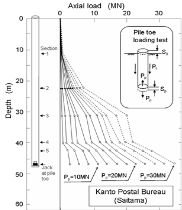
Figure 5 Axial load versus depth in the pile toe loading test at Kanto Postal Bureau (Shibuya et al. 1997)
