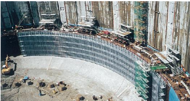
Figure 51 Installation of a block hoop at the depth of -28m
