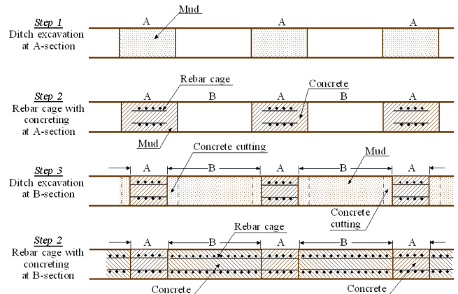
Figure 40 Diaphragm wall by concrete cutting method
