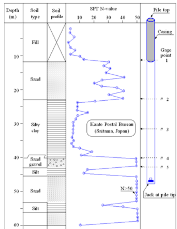
Figure 2 Soil profile at the site of Kanto Postal Bureau (Shibuya et al. 1997)
