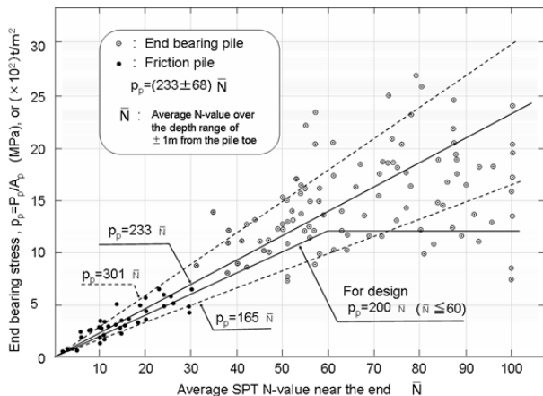
Figure 32 Summary plots of the ultimate toe bearing load intensity as function of averaged N-value (from Japanese manual)
