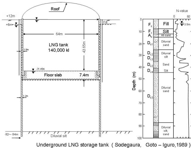
Figure 36 Underground LNG storage tank at Sodegaura (Goto-Iguro, 1989)
