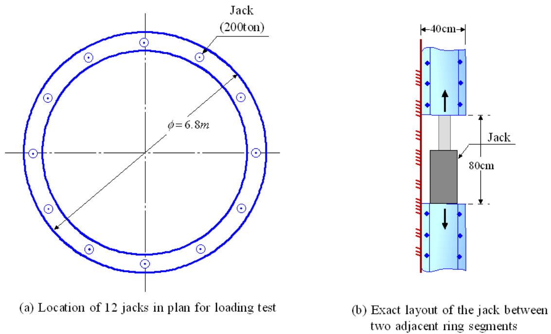
Figure 29 Details of jack installation
