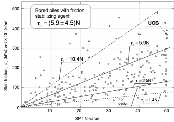
Figure 33 Summary plots of the ultimate skin friction as functions of SPT N-value (from Japanese manual)
