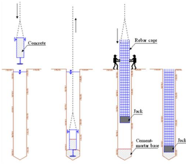
Figure 3 Procedures for installing a jack at the toe of the cast-in-place reinforced concrete pile
