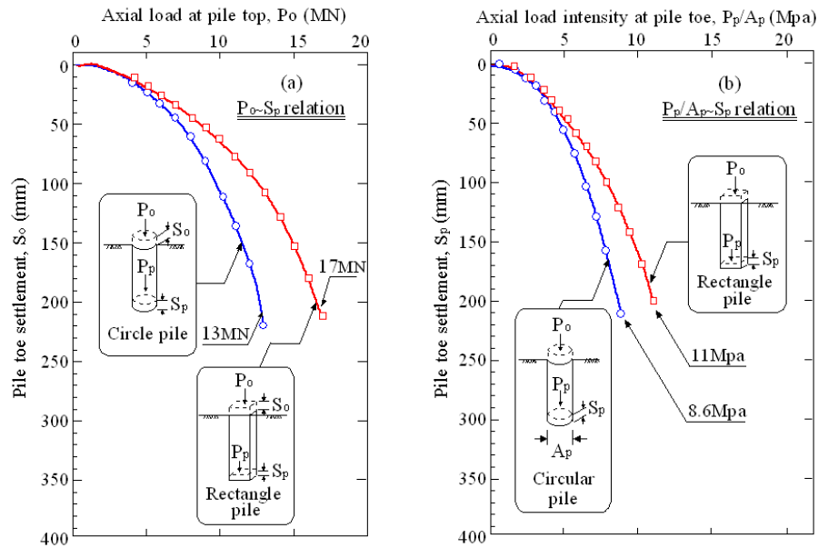
Figure 20 Load-settlement curves from the pile loading tests on the circular and rectangular piles at Tsukimino (Iwanaga et al. 1991)
