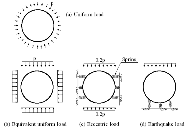
Figure 37 Three types of external loads in the design of the diaphragm wall
