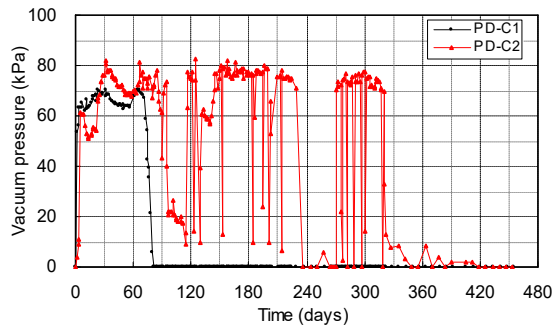
Figure 10 Measured vacuum pressure in PVDs using VCM-DT method (Long et al, 2011)
