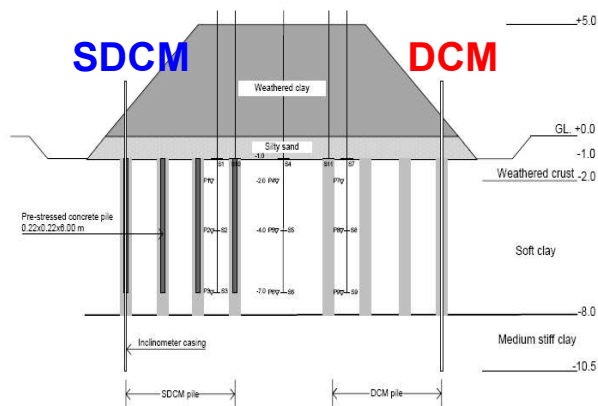
Figure 38 Section view and location of instruments of the SDCM embankment
