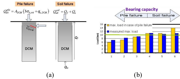
Figure 35 Bearing capacity of DCM piles on soft Bangkok clay (Petchgate et al., 2003)
