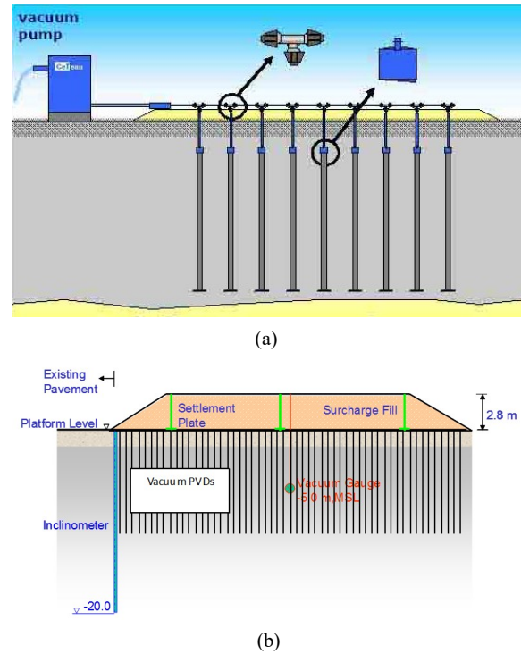
Figure 8 Vacuum PVD by direct connection method: (a) Cross-section and (b) Monitoring instruments
