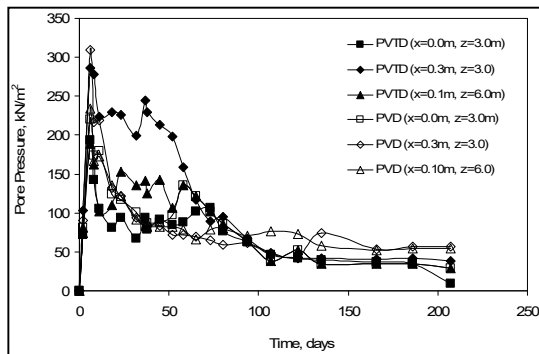
Figure 25 Excess pore pressures for Conventional PVD and Thermal PVD (PVT)
