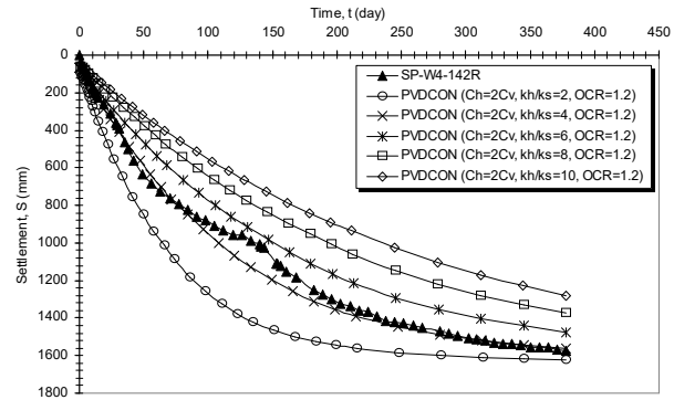
Figure 19 Observed and predicted settlements using PVDCON of Conventional PVD
