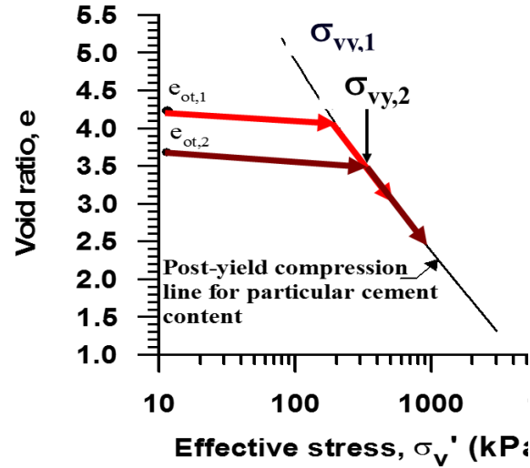
Figure 34 Relation between after curing void ratio and effective stress
