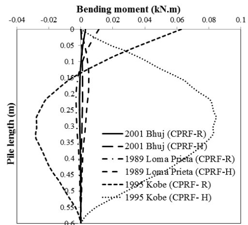
Figure 9 Normalized bending moment profile for different earthquake loads
