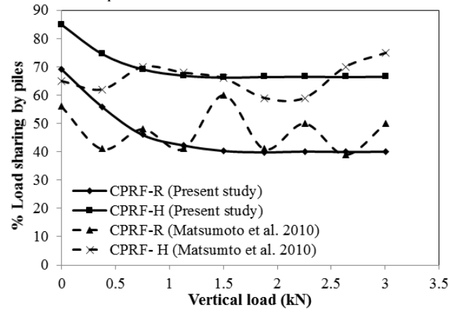
Figure 4 Comparison of load sharing by piles in CPRF as obtained in present study with those reported by Matsumoto et al. (2010)
