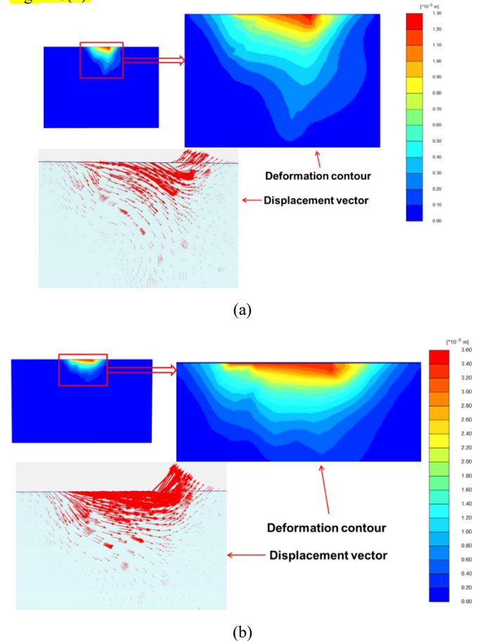
Figure 6 Lateral displacement contour and displacement vector for (a) CPRF-R, (b) CPRF-H under 1995 Kobe earthquake motion simulated as pseudo-static load
