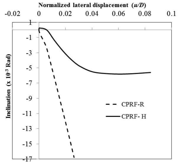
Figure 12 Inclination of raft with normalized lateral displacement for both CPRF connections
