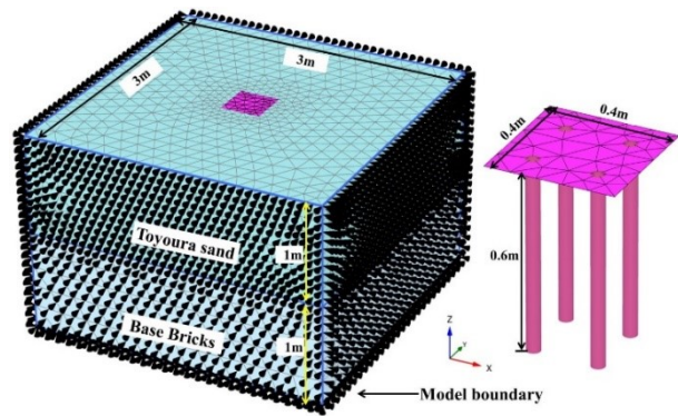
Figure 2 Three-dimensional view of chosen CPRF and soil model in PLAXIS3D
