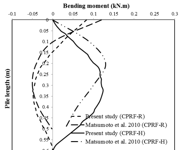
Figure 5 Comparison of bending moment variations along pile length as obtained in present study with those reported by Matsumoto et al. (2010)
