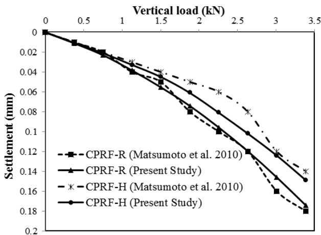
Figure 3 Comparison of load-settlement curves as obtained in present study with those reported by Matsumoto et al. (2010)
