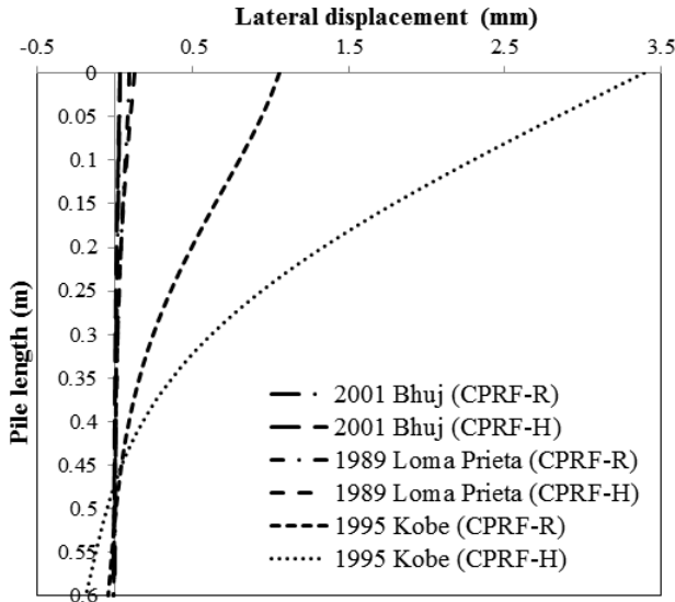
Figure 10 Lateral displacements along pile length for different earthquake loads
