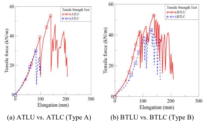
Figure 8 Comparison the tensile test results for test specimen without and with a centre cut wire for Type-A or Type-B mesh panels loaded in the longitudinal direction.
