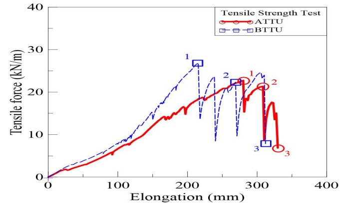
Figure 10 Typical tensile test results for Type A and Type B mesh panels loaded in the transverse direction without one cut wire (ATTU vs. BTU)
