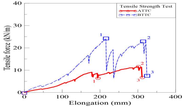
Figure 11 Typical tensile test results for Type A and Type B mesh panels loaded in the transverse direction with one cut wire (ATTC vs. BTTC).
