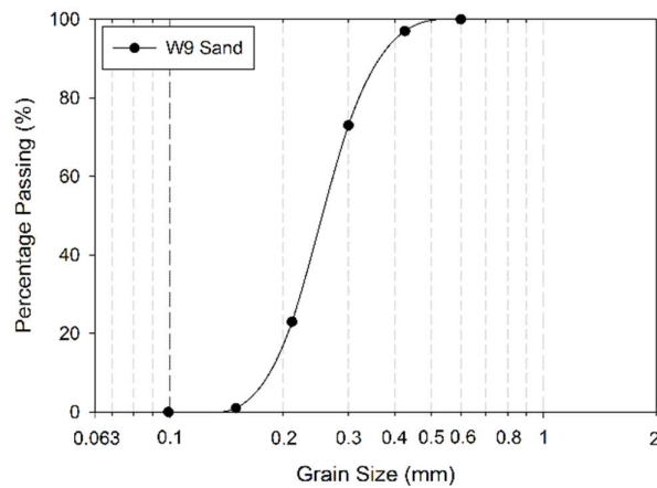
Figure 1 Particle size distribution of admixed sand
