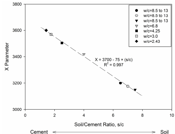
Figure 5 Linear relationship between X parameter and soil:cement ratio
