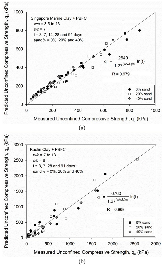
Figure 10 Comparison between predicted and measured unconfined compressive strength of cement-treated clay; (a) Singapore marine clay, (b) Kaolin clay
