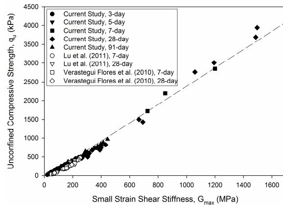
Figure 12 Correlation between unconfined compressive strength ( q_u ) and small-strain shear stiffness ( G_{max} )
