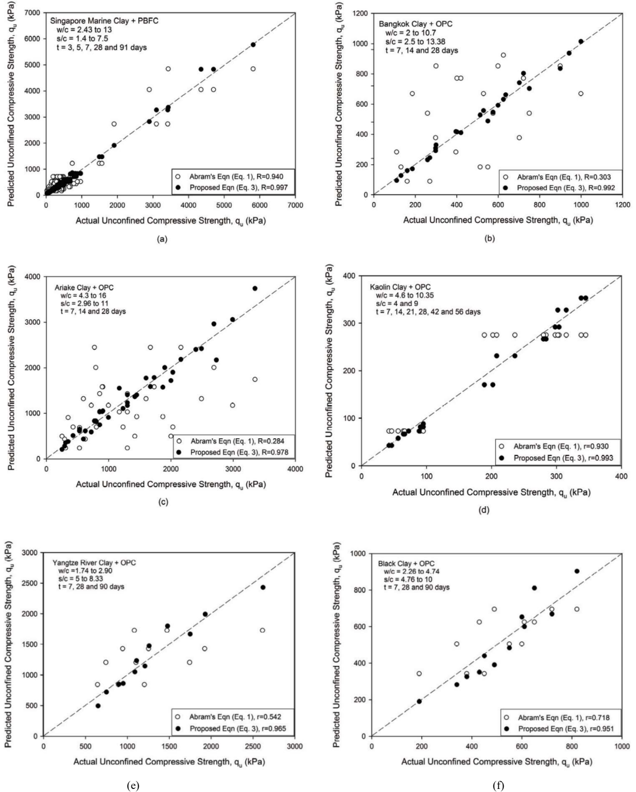
Figure 7 Strength prediction of various clay and cement types at different water:cement, soil:cement ratios, and curing time; (a) Singapore marine clay (Chian et al. 2015a) (b) Bangkok clay (data from Horpibulsuk et al. 2003) (c) Ariake clay (data from Horpibulsuk et al. 2003) (d) Kaolin clay (data from Verástegui Flores et al. 2010) (e) Yangtze river clay (data from Wu et al. 1998) (f) Black clay (data from Chen et al. 2001)
