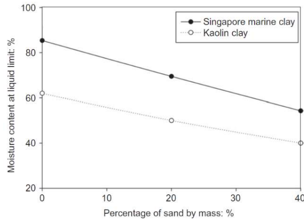
Figure 2 Liquid limit of Singapore marine clay
