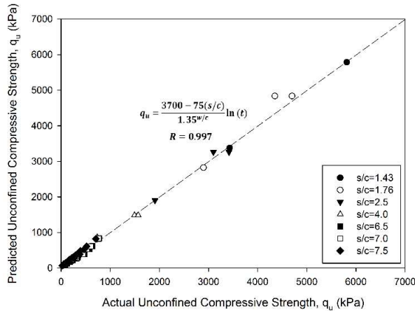
Figure 6 Predicted versus actual unconfined compressive strength with Eq. (3)
