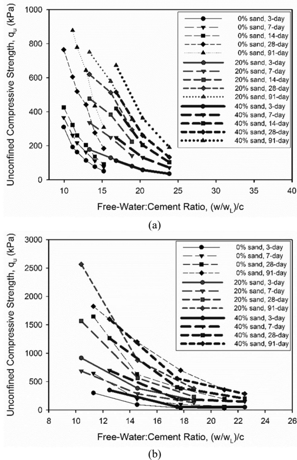
Figure 9 Influence of free water to cement ratio on unconfined compressive strength for cement-treated clay with different sand content and curing duration; (a) Singapore marine clay, (b) Kaolin clay
