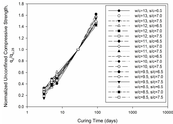
Figure 4 Effect of curing time on normalized unconfined compressive strength
