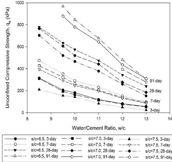
Figure 3 Effect of mixing proportions on unconfined compressive strength of Singapore marine clay
