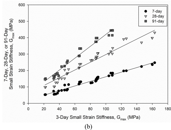
Figure 11 Correlation between early-age (3-day) and later-age (7-day, 28-day and 91-day); (a) unconfined compressive strength, (b) small-strain shear stiffness
