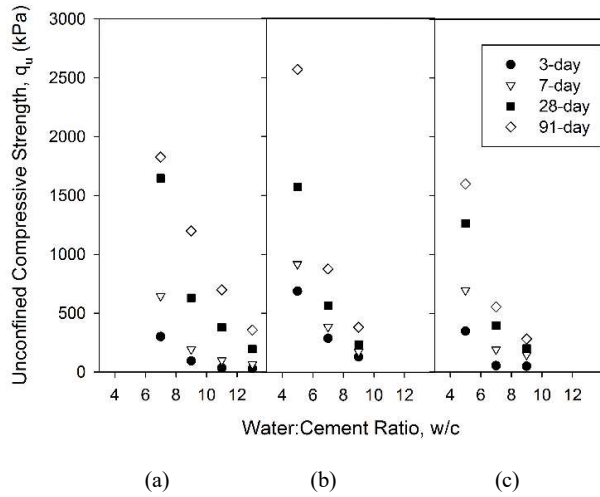
Figure 8 Influence of water to cement ratio on unconfined compressive strength of cement-treated kaolin clay with soil to cement ratio of 7; (a) 0% sand content (b) 20% sand content (c) 40% sand content
