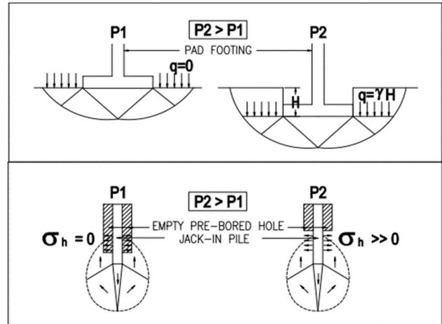
Figure 24 Pressure bulb and plastic zone for shallow foundation and pile foundation
