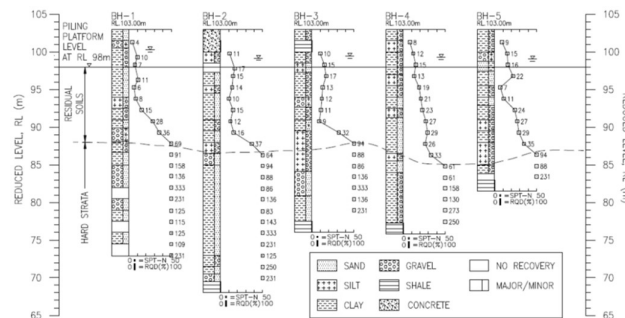
Figure 23 Borehole logs of subsoil profiles
