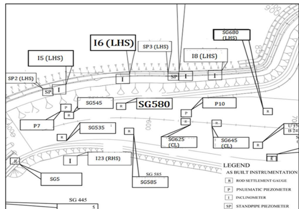
Figure 8 Installed Instrumentations on Embankment
