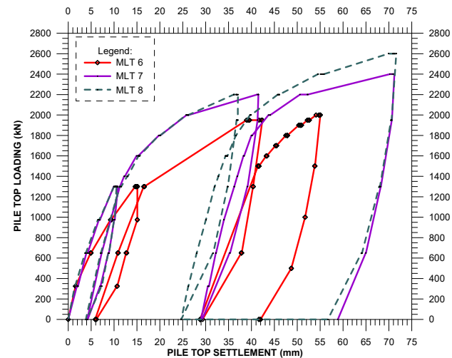
Figure 25 Pile top loading (kN) versus pile top settlement for (a) contractually scheduled MLT results and (b) additional MLT results
