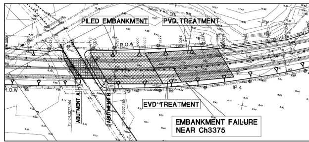
Figure 14 Layout of distressed bridge abutments and embankment
