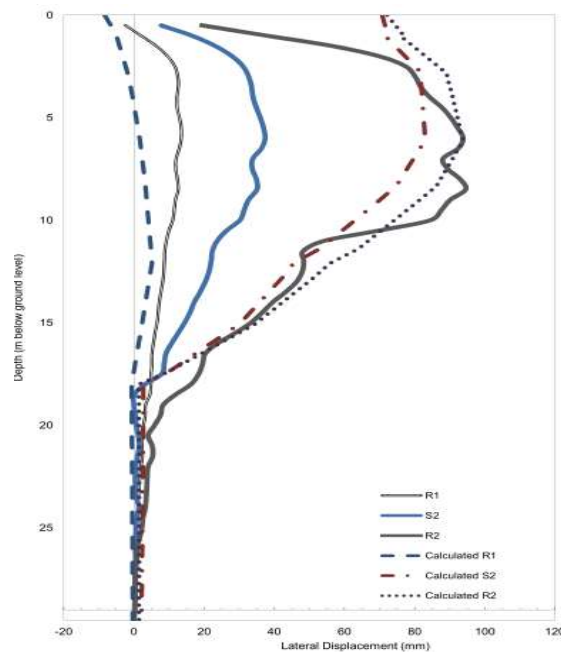
Figure 13 Comparison of Lateral Displacement Profile
