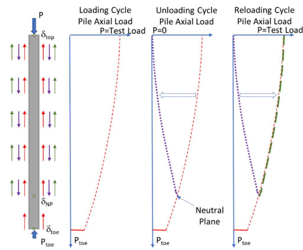
Figure 28 Schematic diagram of Pile Load Test Results
