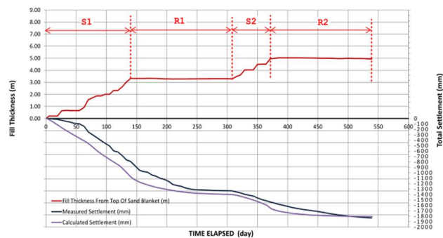
Figure 12 Comparison of Back Analysed Settlement Trend with Actual Measurement
