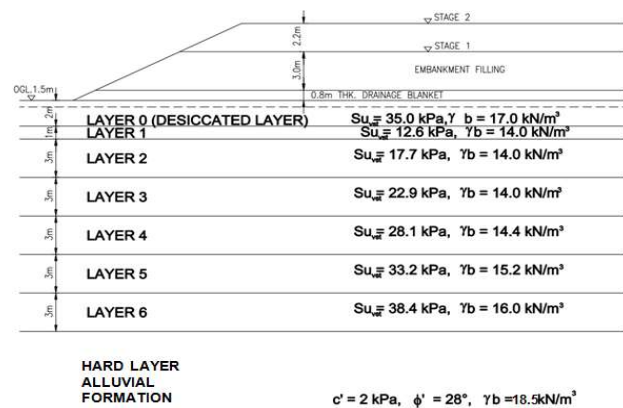
Figure 7 Typical Cross Section of Embankment in Stages
