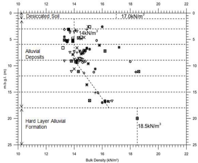
Figure 6 Interpreted Subsoil Bulk Density
