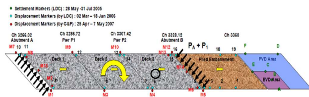
Figure 16 Monitoring layout
