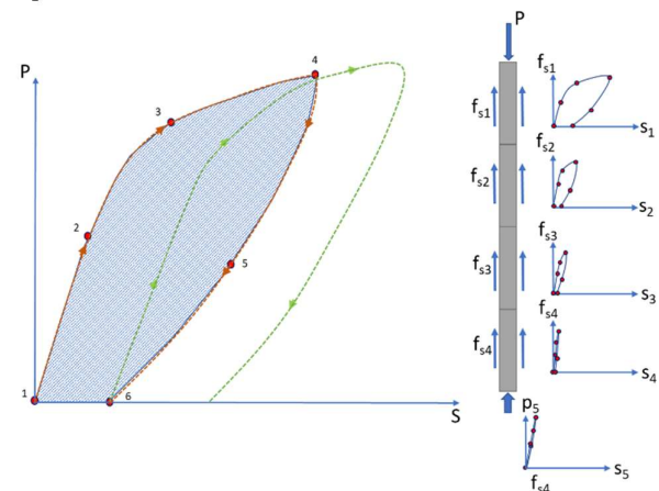
Figure 27 Schematic diagram of Pile Load Test Results
