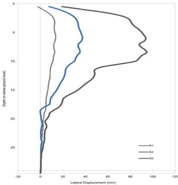
Figure 10 Inclinometer I6 Monitoring Results
