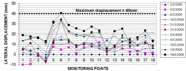
Figure 17 Movements in the longitudinal direction
