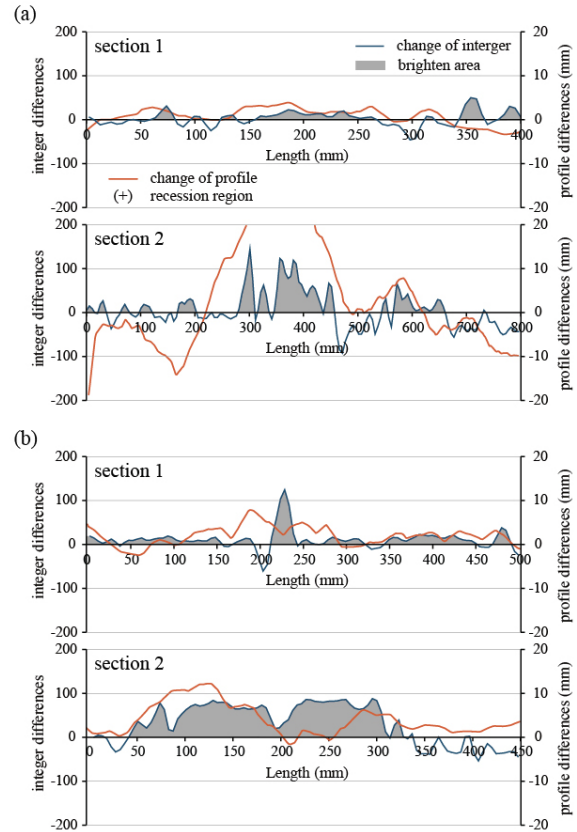
Figure 10 Changes of brightness integers (I) and the loss of roughness of profiles in vertical directions; shale (a), sandstone (b)
