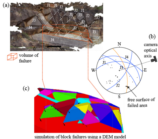
Figure 2 Photogrammetric model for a failed rock slope (a); stereonet projection of main joint sets (b); a 3DEC model at a sliding step (c) (Kim et al., 2015a)
