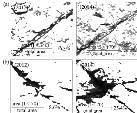
Figure 11 Comparisons of filtered areas by MATLAB threshold technique over the two year interval; shale section 2 (a), sandstone section 2 (b)
