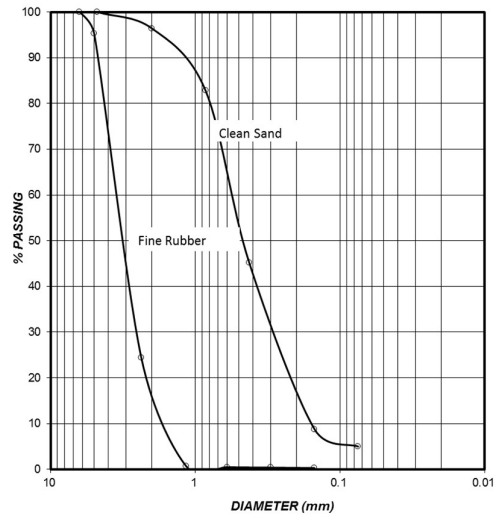
Figure 1 Grain Size Distribution Curves
