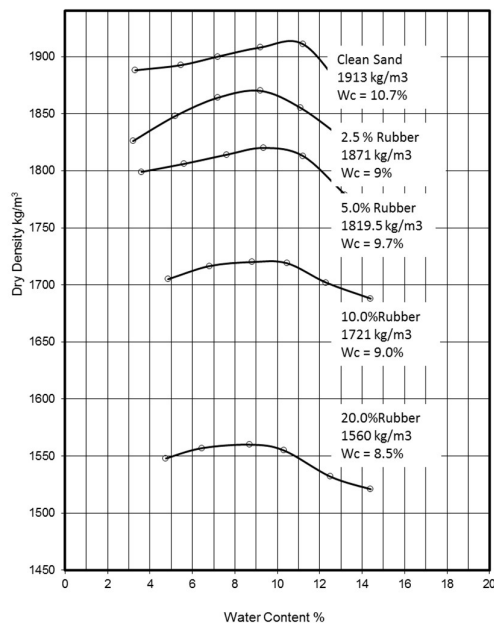
Figure 2 Compaction Test Results
