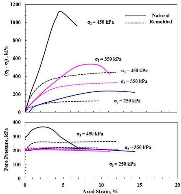
Figure 4 Stress and pore-water pressure versus axial strain for naturally cemented and remolded specimens, Depth = 2 m
