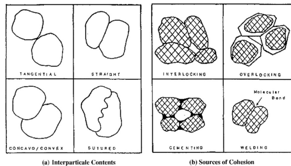
Figure 8 Types of interparticle contact and main sources of cohesion in cohesive sands (Barton 1993)
