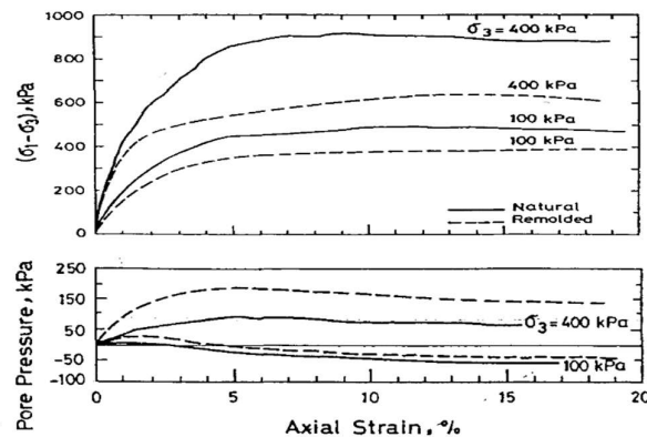
Figure 2 Stress and pore-water pressure versus axial strain for naturally cemented and remolded specimens, Depth = 0.3 m (Ismael 1999)
