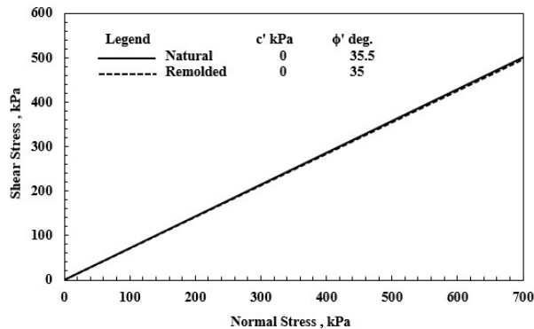
Figure 7 Failure envelopes for naturally cemented and remolded specimens, Depth = 4 m
