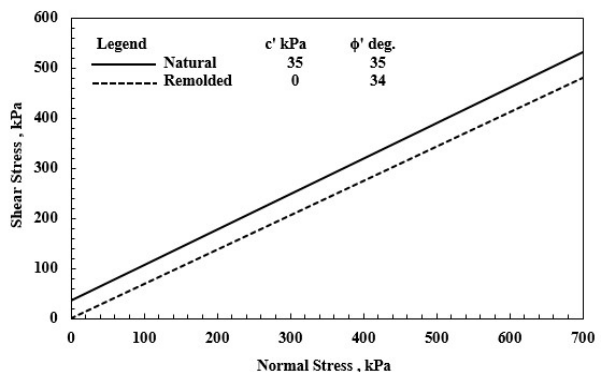
Figure 5 Failure envelopes for naturally cemented and remolded specimens, Depth = 2 m
