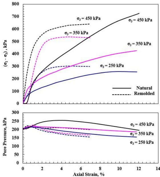
Figure 6 Stress and pore-water pressure versus axial strain for naturally cemented and remolded specimens, Depth = 4 m
