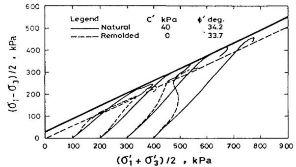
Figure 3 Effective stress path and failure envelope for naturally cemented and remolded specimens, Depth = 0.3 m (Ismael, 1999)
