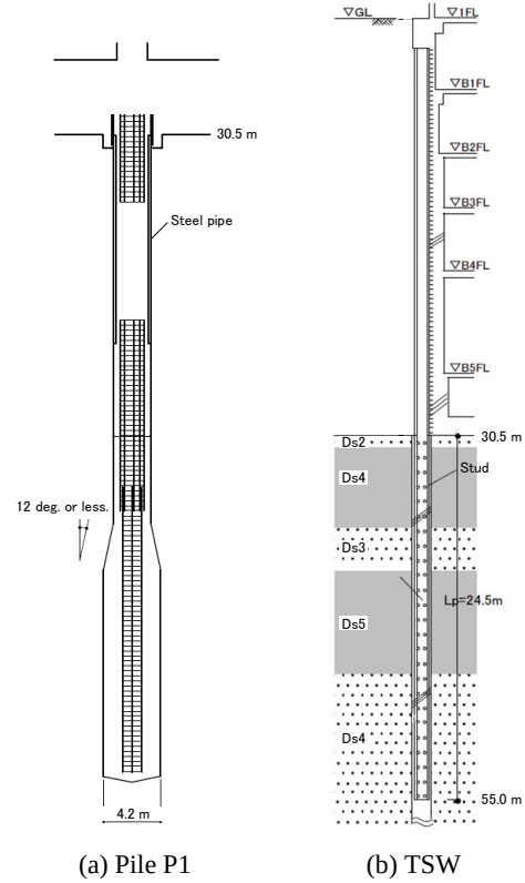
Figure 7 Cross-section of cast-in-place concrete pile and TSW
