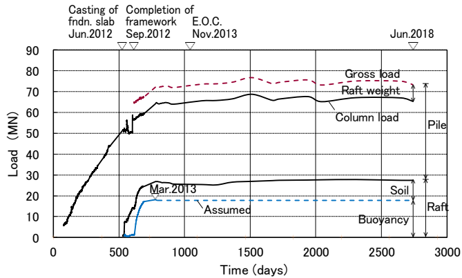
Figure 14 Load sharing between pile and raft in the tributary area of Column 4F
