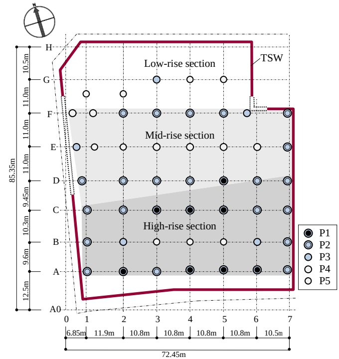
Figure 4 Foundation plan with layout of piles and TSW
