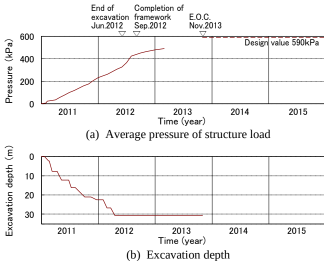
Figure 10 Structure load and excavation depth vs. time
