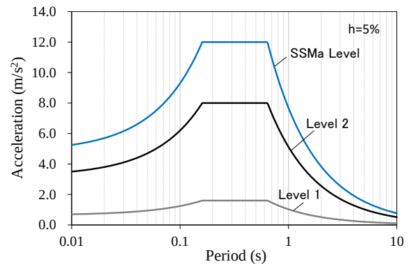
Figure 6 Acceleration response spectra on bedrock.
