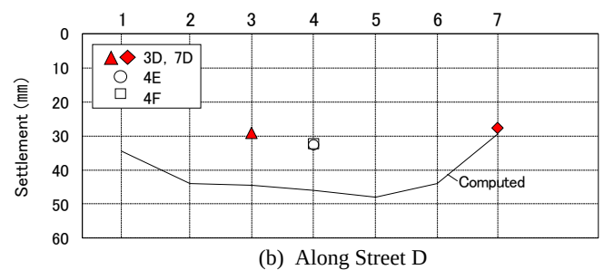
Figure 12 Measured and computed settlement profiles at 1st floor (Feb. 22, 2013)
