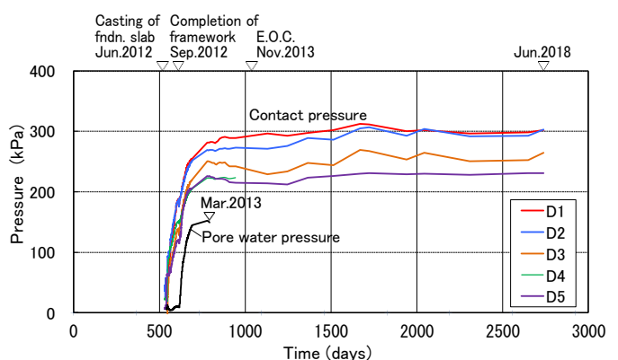
Figure 13 Measured contact pressure and pore-water pressure underneath the raft
