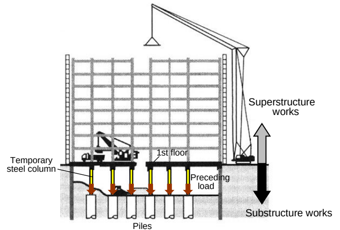
Figure 8 Schematic of top-down method
