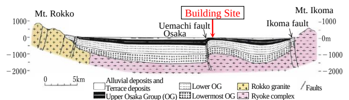
(b) East-west section of geological profile (Section A-A')
