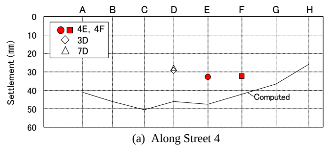
Figure 11 Measured vertical ground displacements in reference to the depth of 74.9 m
