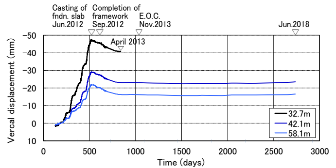
Figure 11 Measured vertical ground displacements in reference to the depth of 74.9 m
