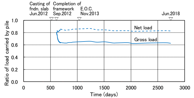
Figure 15 Ratio of load carried by pile after casting of raft
