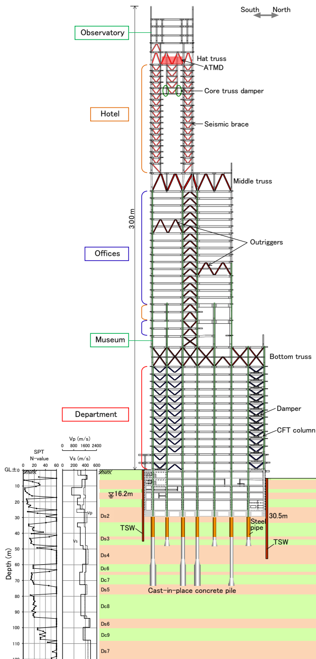
Figure 3 Cross-section of building and foundation (Street 5)
