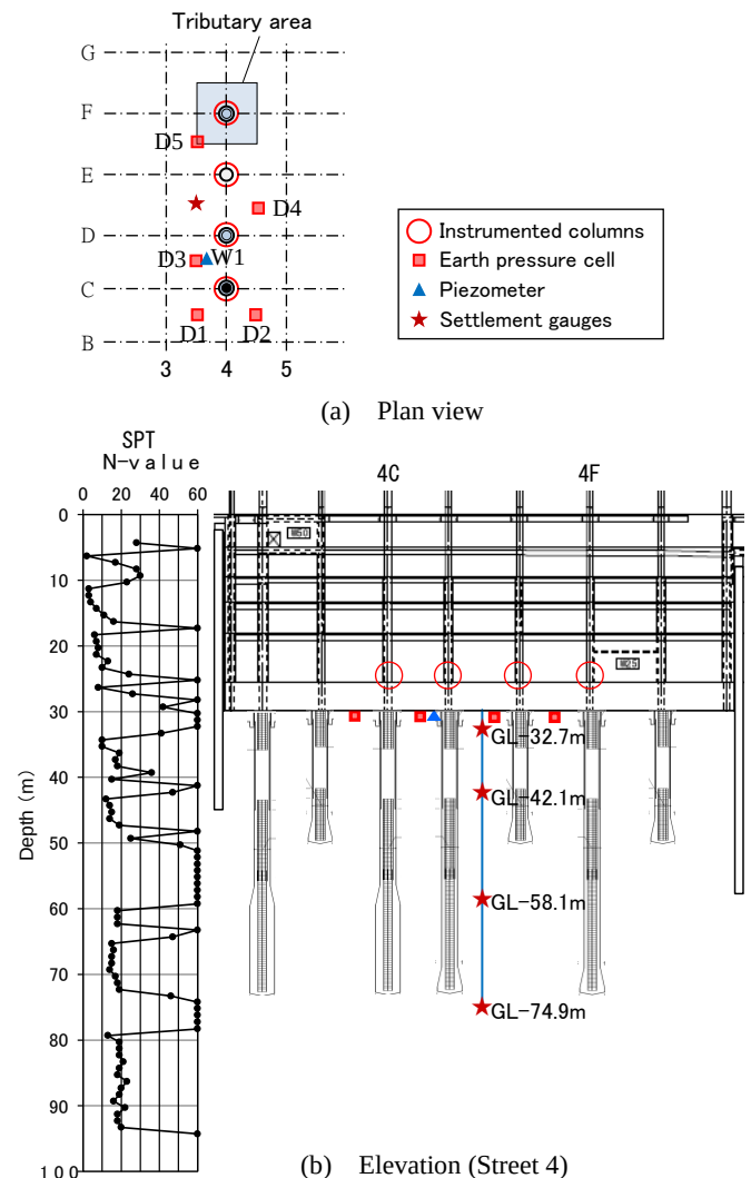
Figure 9 Location of monitoring devices
