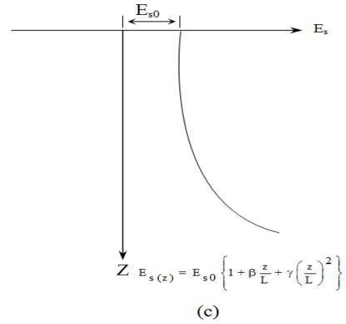
Figure 4 Definition Sketch (a) Non-homogeneous end bearing granular pile, (b) Variation of Modulus of deformation with depth for pile, (c) Variation of Modulus of deformation with depth for soil.
