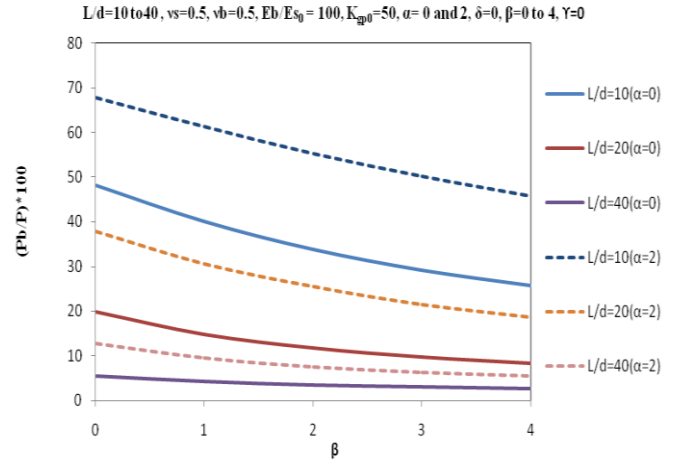
Figure 31 Variation of the percentage base load with non-homogeneity parameter, \beta ( K_{gp0}=50 )
