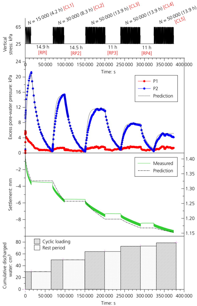
Figure 14 (a) applied stress; (b) EPWP; (c) settlement or void ratio; (d) volume of water discharged (CL – cyclic loading stages; RP – rest periods) (after Atapattu et al., 2023, with permission from Emerald Publishing Ltd.)
