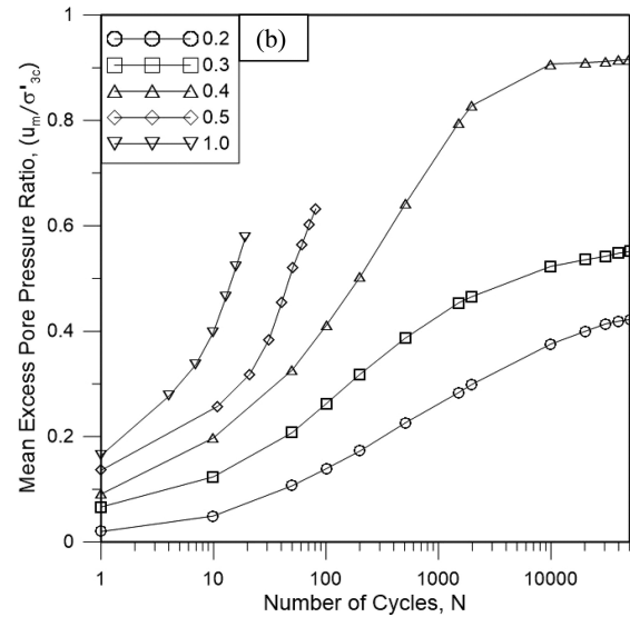
Figure 2 Effect of CSR on axial strains and mean excess pore water pressure ratio (after Indraratna et al. 2020a, with permission from Canadian Science Publishing)
