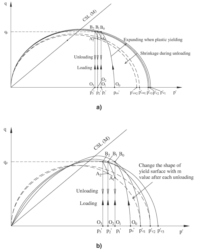
Figure 15 (a) Illustration of Ni et al. (2015) model; (b) Illustration of Truong et al. (2021) model (adopted from Indraratna et al., 2021, with permission from Elsevier)
