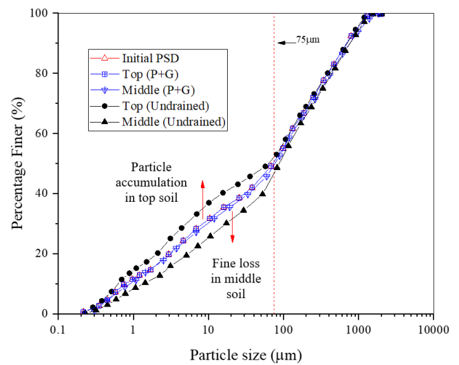
Figure 9 Particle size distribution – Undrained (U) and cyclic tests with PVD-Geocomposite system (P+G) (Arivalagan et al., 2022, with permission from Geotextiles and Geomembranes)
