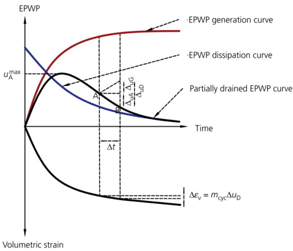
Figure 11 EPWP behaviour under partially-drained loading (adopted from Atapattu et al., 2023, with permission from Emerald Publishing Ltd.)
