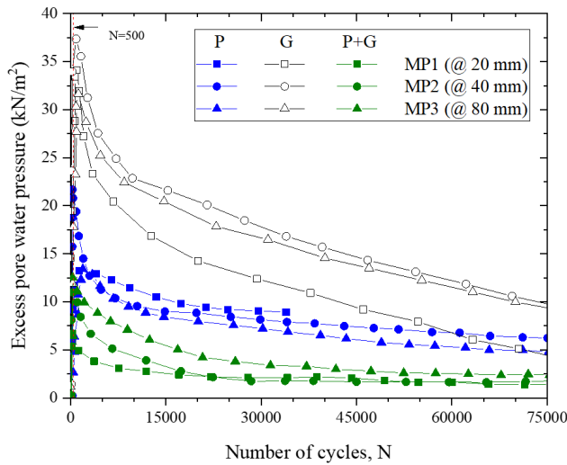
Figure 7 Development of excess pore water pressure – Tests with PVDs (P), Geocomposites (G) and PVD-Geocomposite system (P+G) (Arivalagan et al., 2022, with permission from Geotextiles and Geomembranes)
