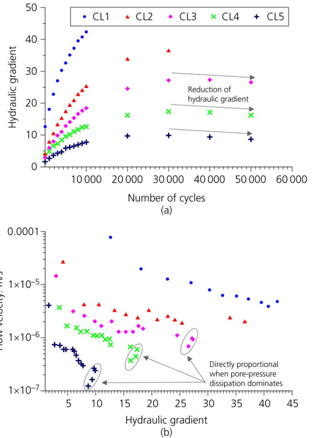
Figure 12 (a) Measured hydraulic gradient during cyclic consolidation test; (b) Relationship between flow rate and hydraulic gradient (after Atapattu et al., 2023, with permission from Emerald Publishing Ltd.)
