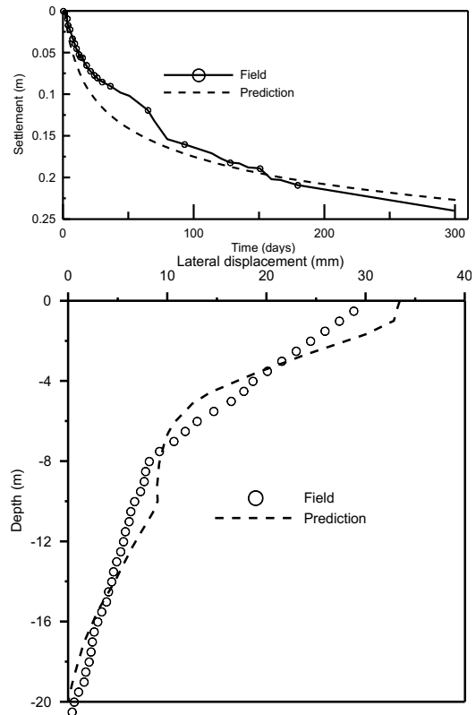
Figure 18 (a) Predicted and measured at the centre line of rail tracks; (b) Measured and predicted lateral displacement profiles near the rail embankment toe at 180 days (after Indraratna et al., 2010, with permission from ASCE)
