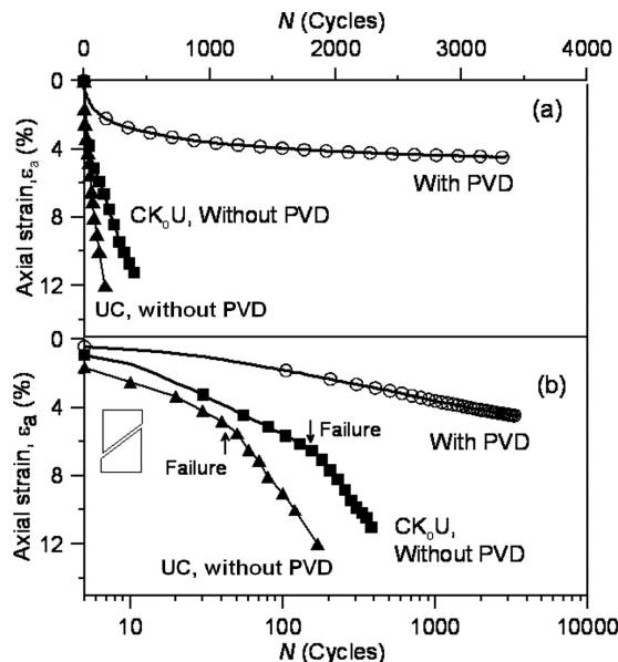
Figure 5 Measured axial strains in undrained (without PVD) and with PVD samples; (a) Number of loading cycles ( N ) in arithmetic scale; (b) N in log scale (after Indraratna et al. 2009, with permission from ASCE)
