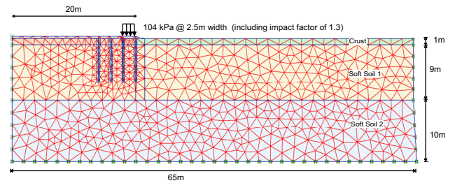
Figure 17 Vertical cross section of rail track foundation (after Indraratna et al., 2010, with permission from ASCE)
