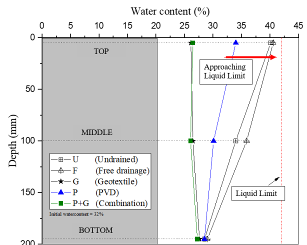
Figure 10 Water content at 100,000 cycles – Test with and without geosynthetics (Arivalagan et al. 2022, with permission from Geotextiles and Geomembranes)
