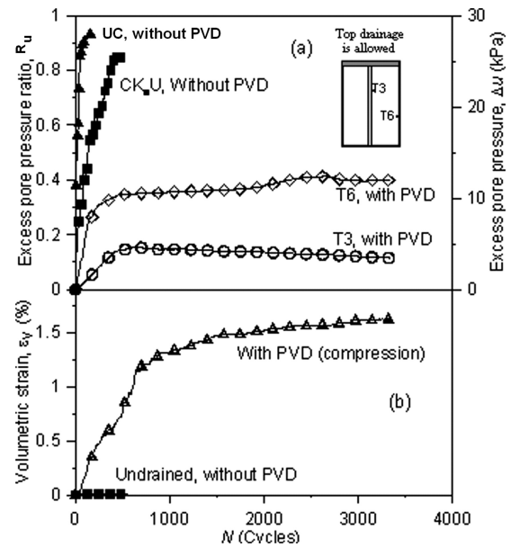
Figure 4 Measured EPWP in undrained (without PVD) and with PVD samples; (a) R_u versus the number of loading cycles ( N ) ; (b) volumetric strains (Indraratna et al., 2009)
