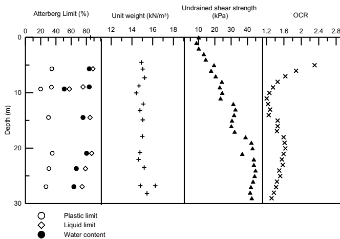
Figure 16 Soil properties at Sandgate Rail Grade Separation Project (adopted from Indraratna et al., 2010, with permission from ASCE)
