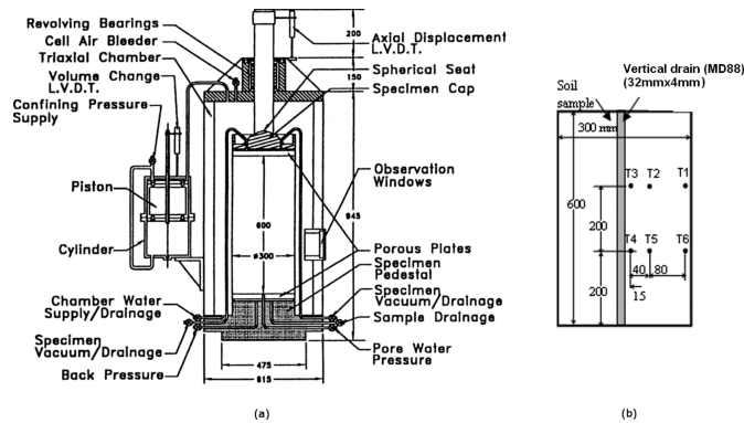
Figure 3 E(a) Schematic diagram of large-scale triaxial apparatus ; (b) locations of miniature pore pressure sensors (after Indraratna et al., 2009, with permission from ASCE)
