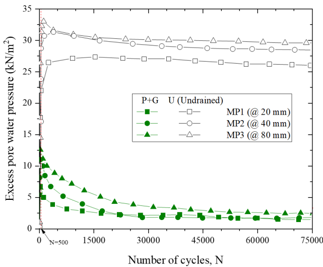
Figure 8 Generation of EPWPs – Undrained (U) and cyclic tests with PVD-Geocomposite system (P+G) (Arivalagan et al., 2022, with permission from Geotextiles and Geomembranes)
