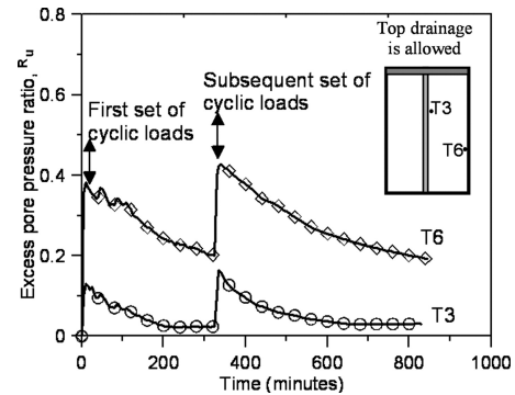
Figure 13 EPWP dissipation during the rest period (after Indraratna et al., 2009, with permission from ASCE)
