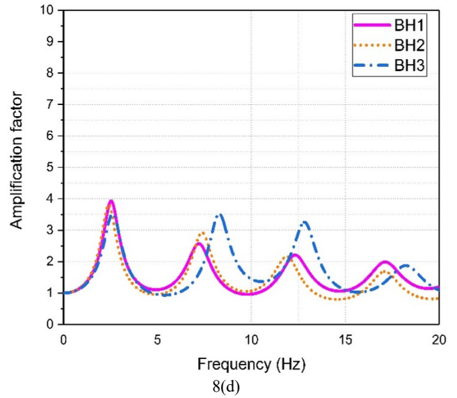
Figure 8 Amplification factor a) Abburaju Palem b) Amaravati c) Nekkallu d) Velagapudi
