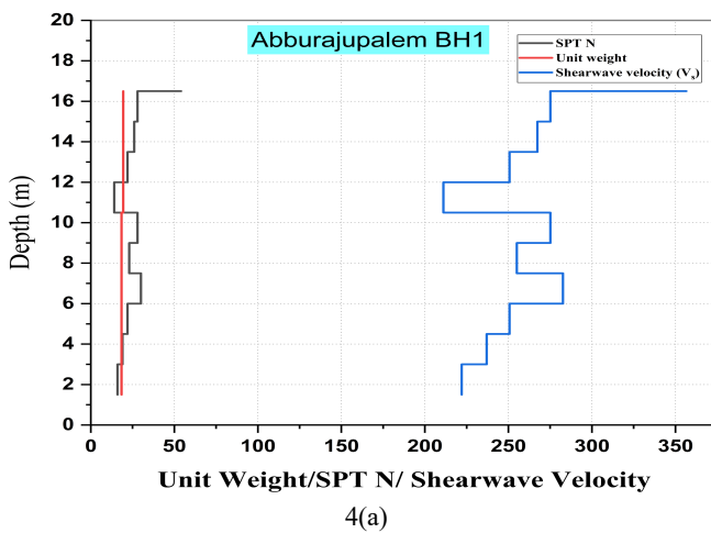
Figure 4 Soil profiles equipped by Unit weight, SPT N, Shear wave velocity and depth of soil a) Abburaju palem b) Amaravati c) Nekkallu d) Velagapudi
