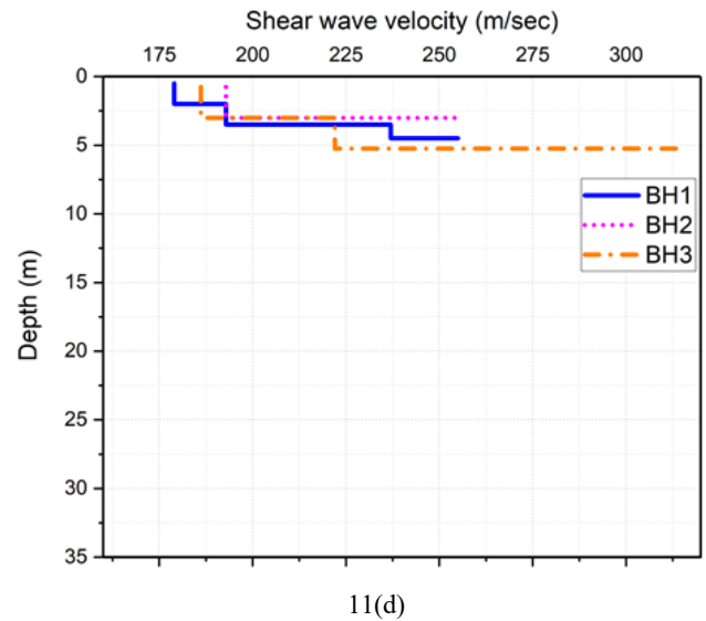
Figure 11 Variation of shearwave velocity with depth a) Abburaju Palem b) Amaravati c) Nekkallu d) Velagapudi
