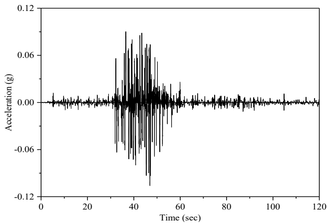
Figure 5 2001 Bhuj earthquake motion
