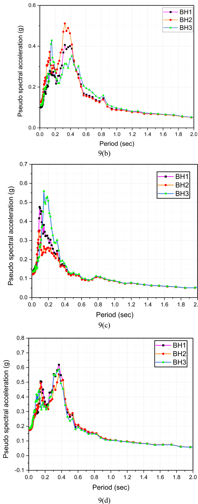
Figure 9 Response spectrum a) Abburaju Palem b) Amaravati c) Nekkallu d) Velgapudi
