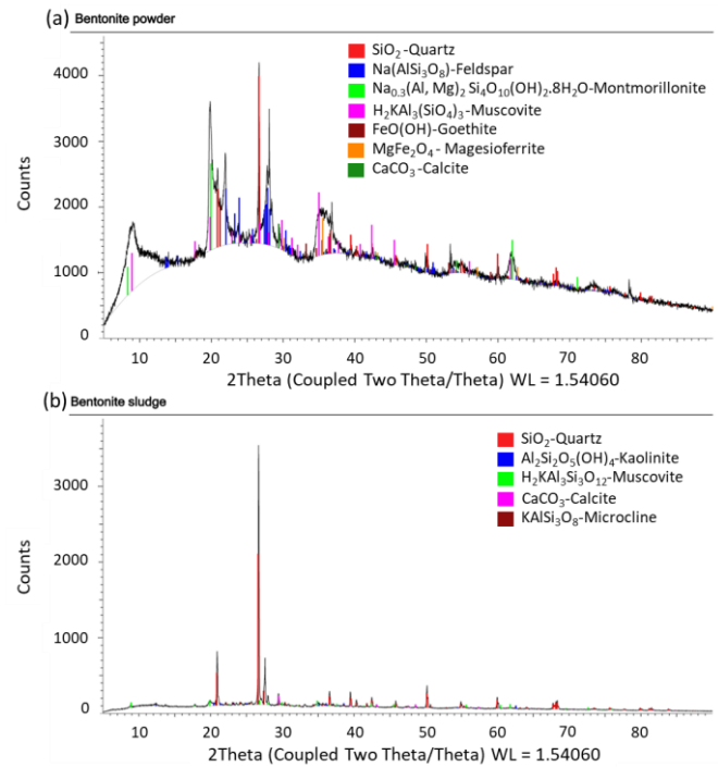
Figure 2 Results of XRD for: (a) BP and (b) BS, with presence of montmorillonite peak (green color)
