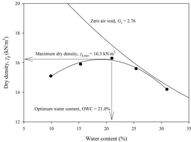
Figure 4 Compaction results for BS
