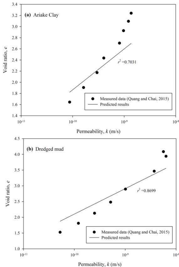
Figure 8 Verified predicted model using results from Quang and Chai 2015 for (a) Ariake clay and (b) Dredged mud
