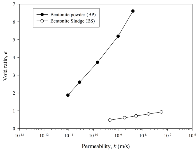
Figure 5 Plot of calculated k versus e values for BP and BS
