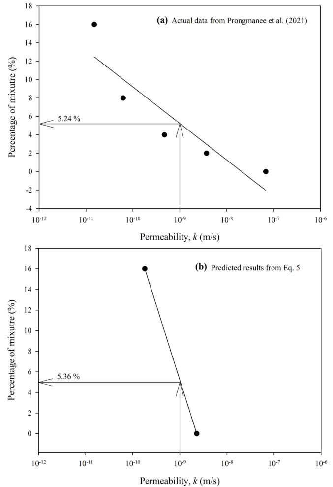
Figure 9 Percentage of mixture versus k value (a) Actual data and (b) Predicted result
