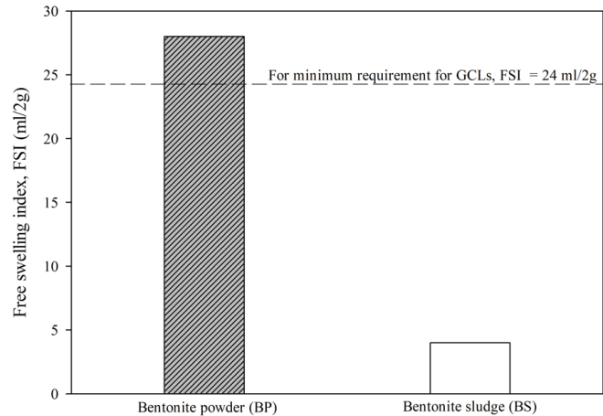
Figure 3 Results of FSI for BP and BS submerged in deionized water
