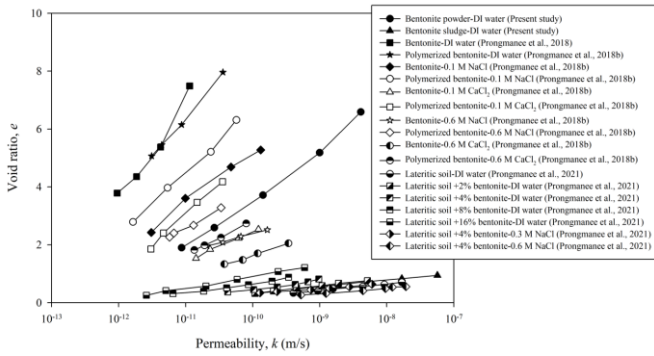
Figure 6 Plot of calculated k versus e values for BP and BS
