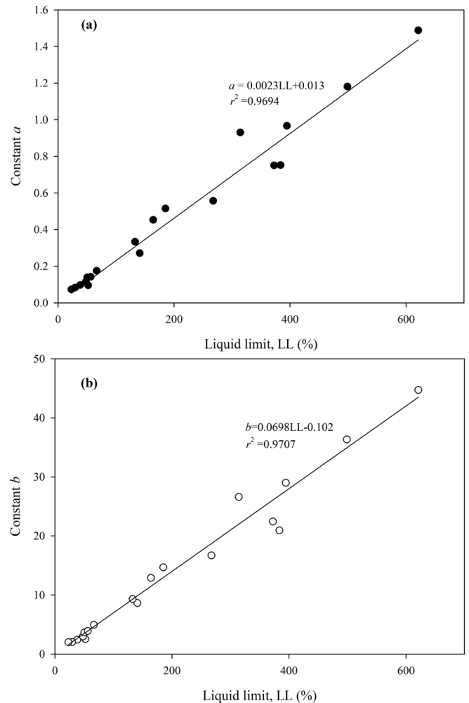
Figure 7 (a) Relationship between LL and constant “ a ” and (b) relationship between LL and constant “ b ”
