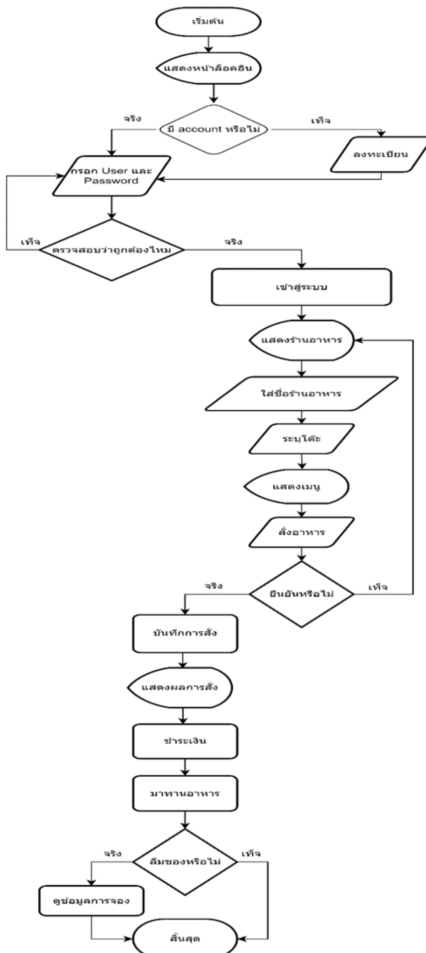
Figure 2. Website workflow diagram
