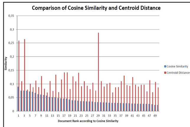
Figure 4. Cosine similarity vs. centroid distance measure (topic: business-related statistics and strategies)
