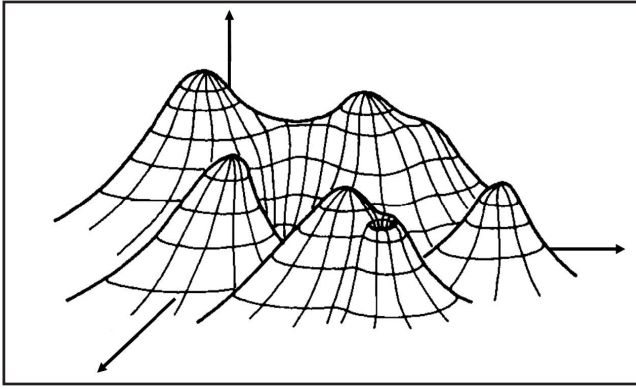
Figure 1. Multimodal distribution density (according to [8])
