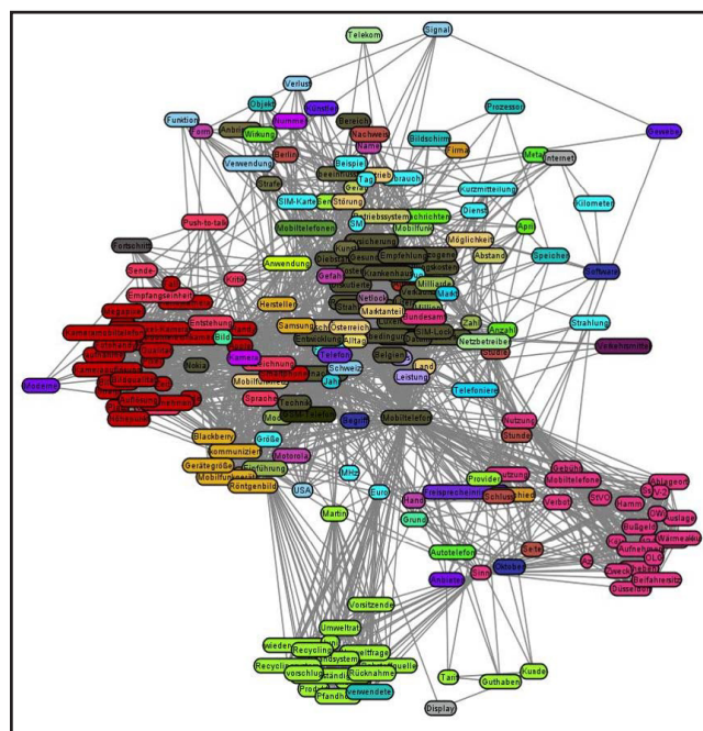
Figure 3. Term clusters of the German Wikipedia entry "Mobiltelefon" created by the Chinese Whispers algorithm
