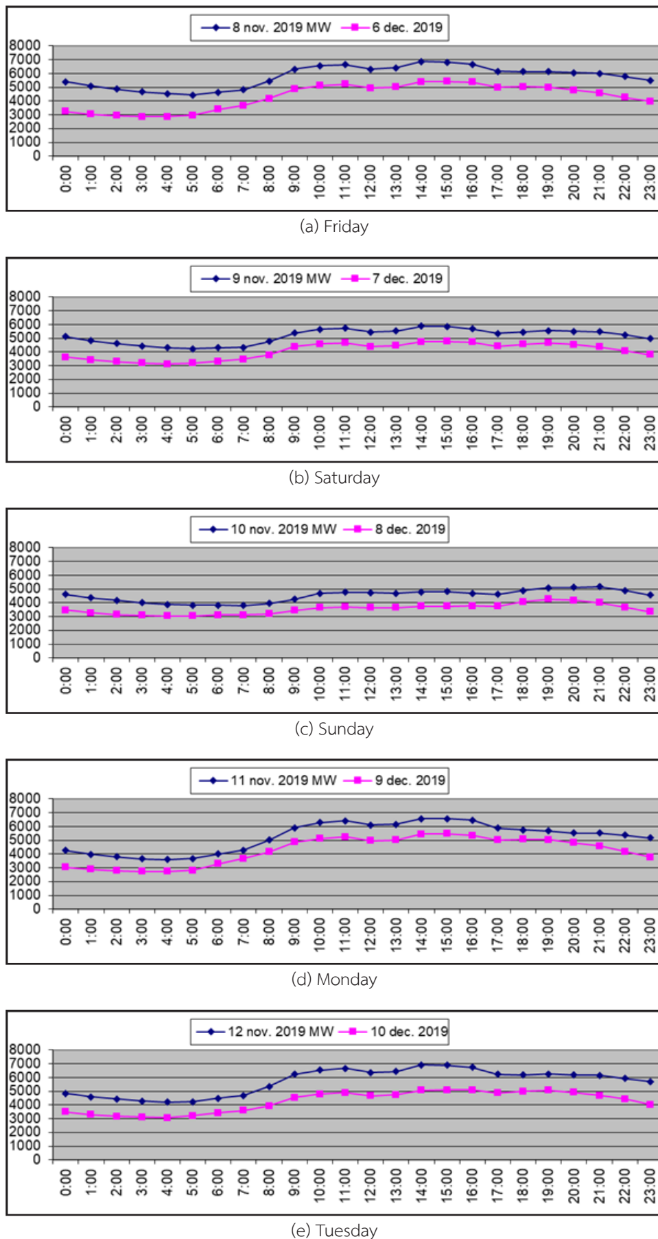
Figure 3. Electrical consumption in Bangkok area comparison between November 8th-12th (warm climate) and December 6th-10th (cold climate), 2019. During working days from Friday to Tuesday have shown in (a), (d), and (e) respectively, while Saturday and Sunday is (b) and (c).
